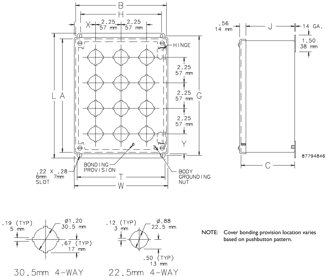
Hole Arrangement
