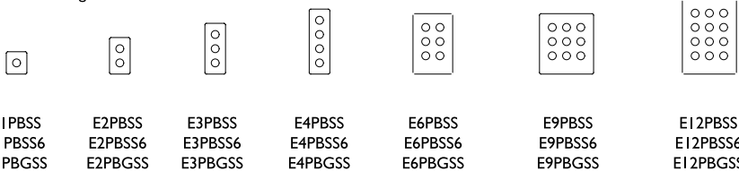
Hole Arrangement
