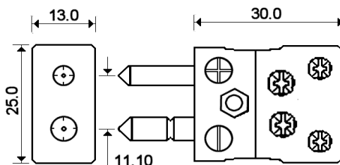
FAR059/0613 JIS Standard Quick Wire Plugs
