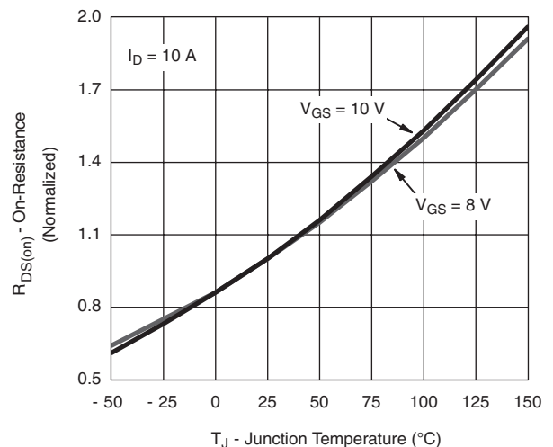
I_D = 10\text{ A} V_{GS} = 10\text{ V} V_{GS} = 8\text{ V} On-Resistance vs. Junction Temperature
