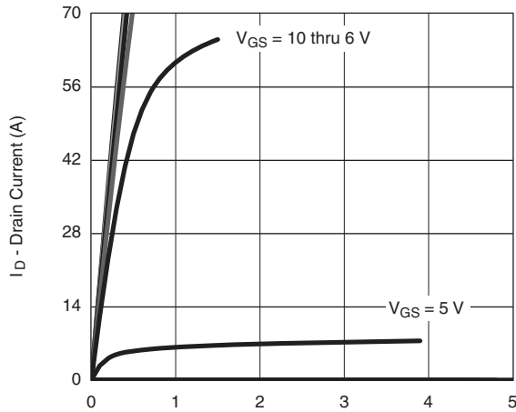
V_{GS} = 10 thru 6 V V_{GS} = 5 V Output Characteristics
