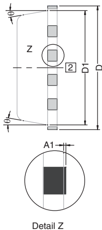
Detail Z
