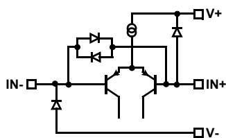
CIRCUIT 1
