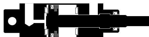
Magnetic piston
