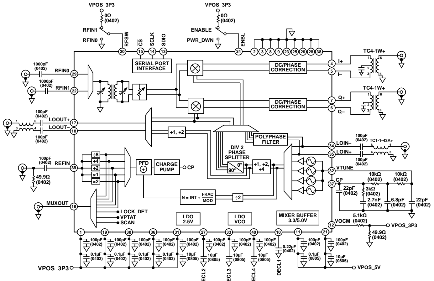
Figure 33. Basic Connections
