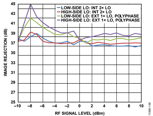
Figure 51. Image Rejection vs. RF Signal Level, f_{IF} = 200 MHz, for High-Side LO Injection f_{LO} = 2000 MHz and f_{RF} = 1800 MHz and Vice Versa for Low-Side Injection
