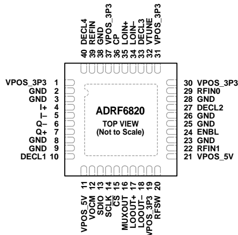
Figure 3. Pin Configuration
