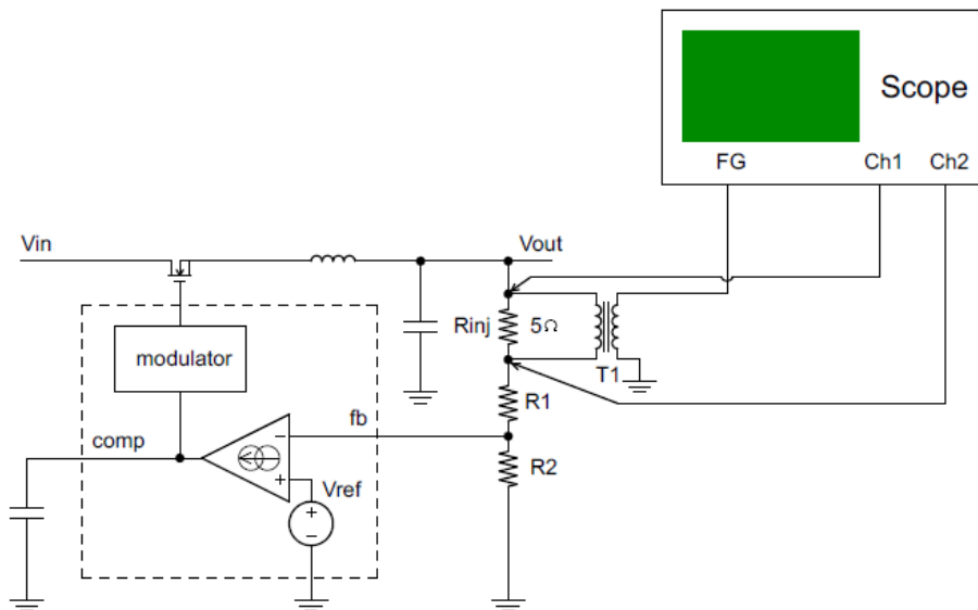
Figure 11. Power supply closed loop feedback network and oscilloscope connections for a Control Loop Response test.
