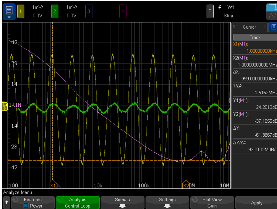
Figure 12. Control Loop Response gain measurement using an InfiniiVision X-Series oscilloscope.
