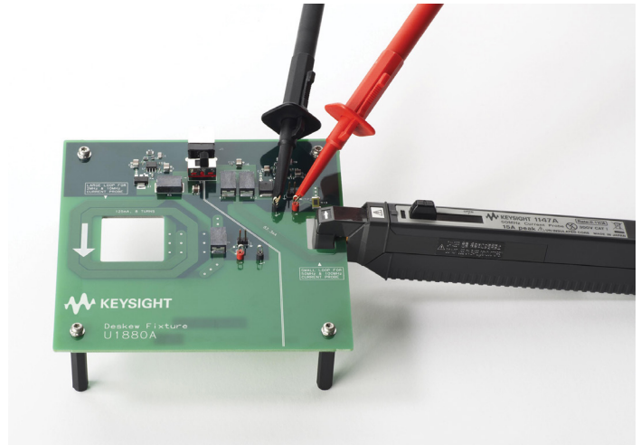
Figure 14. The Keysight U1880A deskew fixture allows you to quickly deskew your voltage and current probes, enabling accurate and precise measurements of power supply efficiency.
