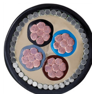
Cross-section of a steel wire armoured cable
