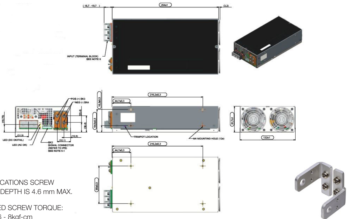
Bus bar adapter (option)
