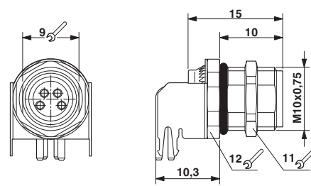
Dimensioned drawing
