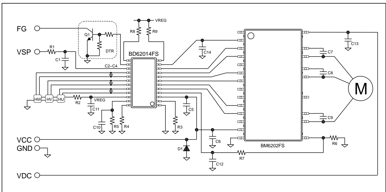
Figure 1. Application circuit example - BD62014FS & BM6202FS
