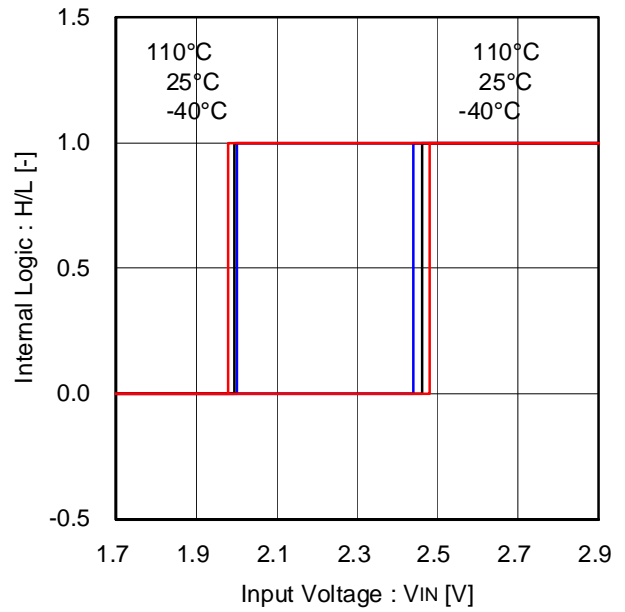
Figure 26. Input threshold voltage (FGS)
