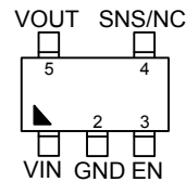
SC-70-5
