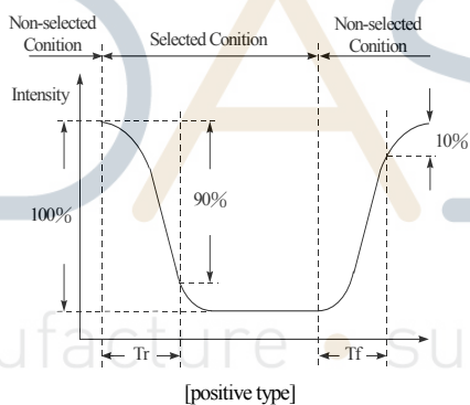
Definition of Response Time ( Tr , Tf )
