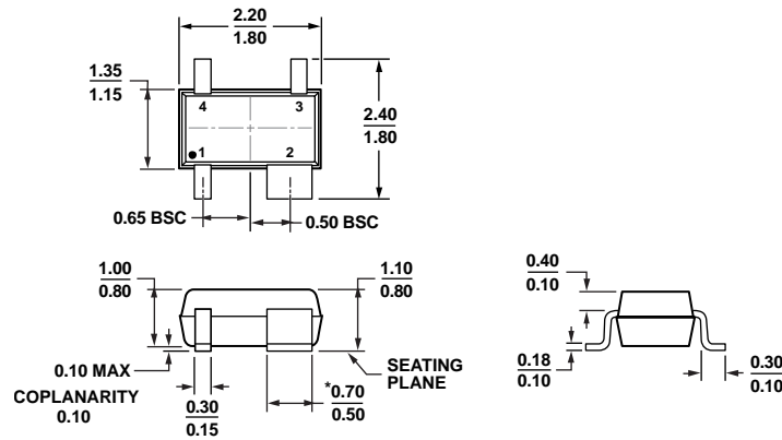
Figure 22. 4-Lead Thin Shrink Small Outline Transistor Package [SC70] (KS-4) Dimensions shown in millimeters
