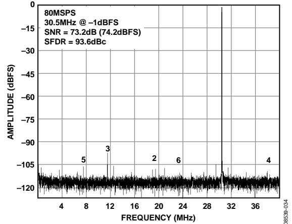
Figure 7. AD9649-80 Single-Tone FFT with f_{IN} = 30.5 MHz
