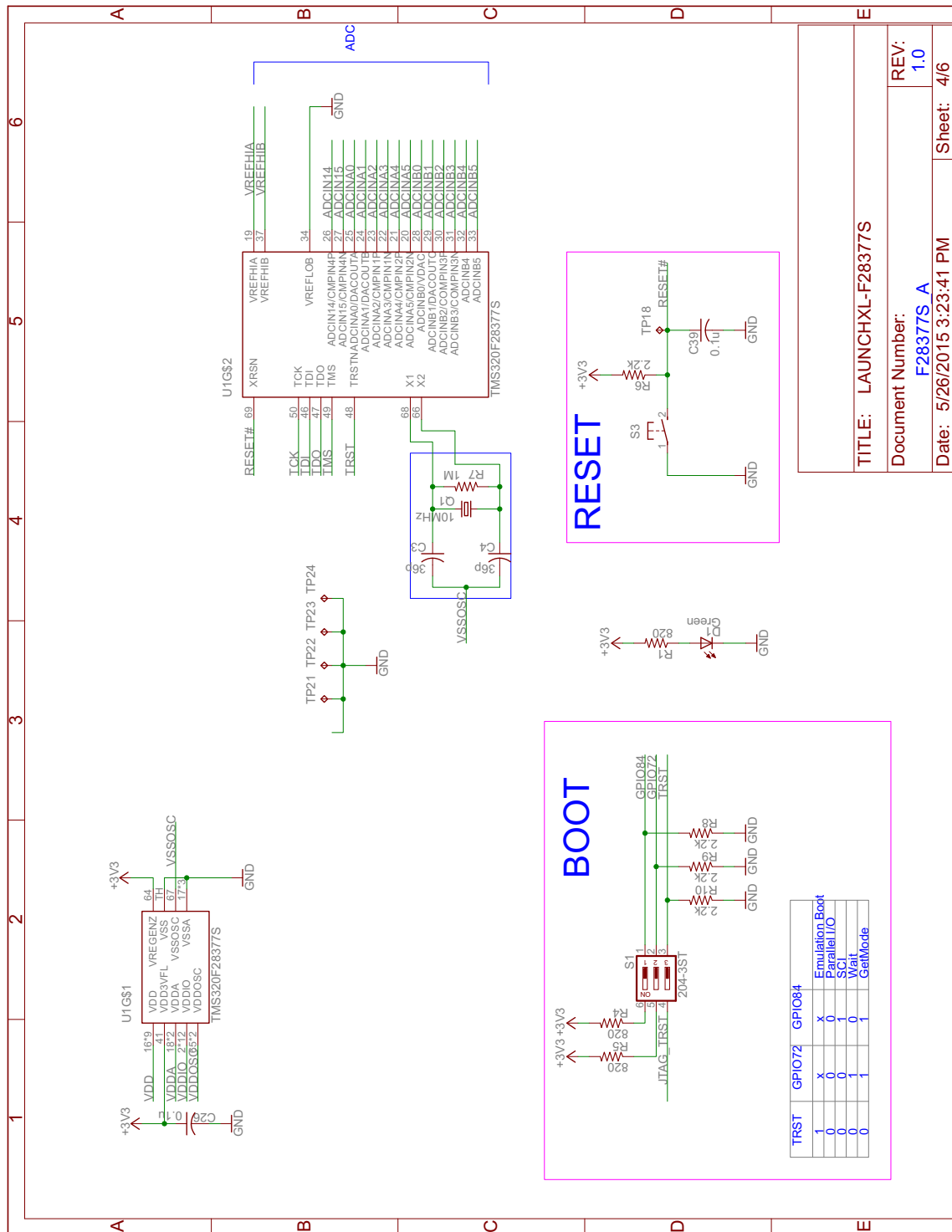
Figure 5. LAUNCHXL-F28377S_A Schematic
