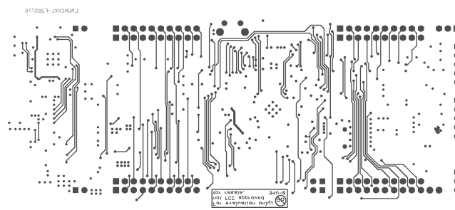
Figure 13. Bottom Copper
