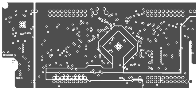
Figure 11. Inner Copper 2
