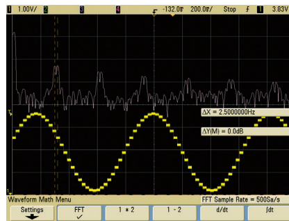
FFT allows you to view the spectral content of this unfiltered sine wave.
