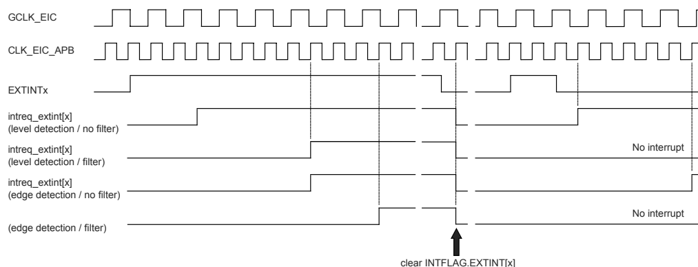
Figure 26-2 Interrupt Detections
