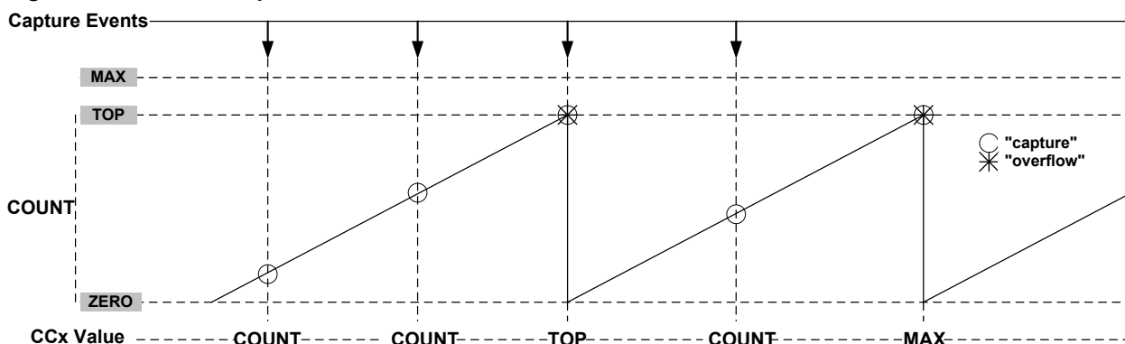
Figure 34-14 Time-Stamp
