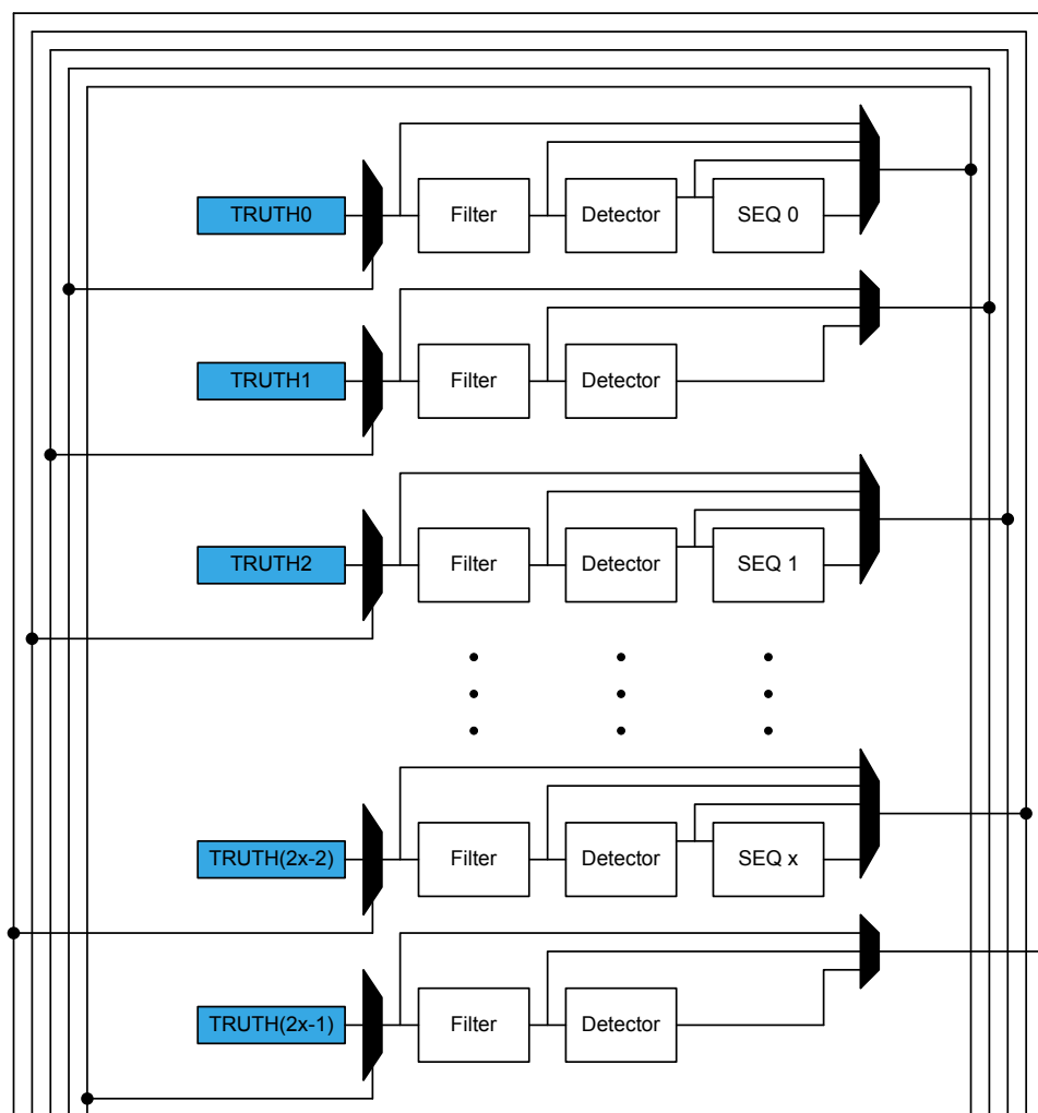
Figure 39-5 Linked LUT Input Selection
