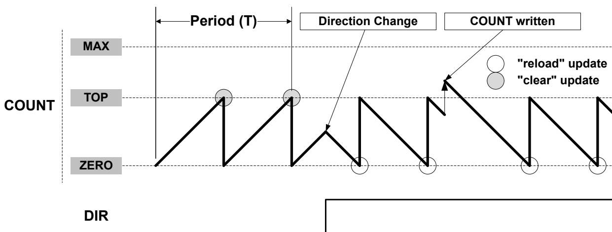
Figure 34-3 Counter Operation
