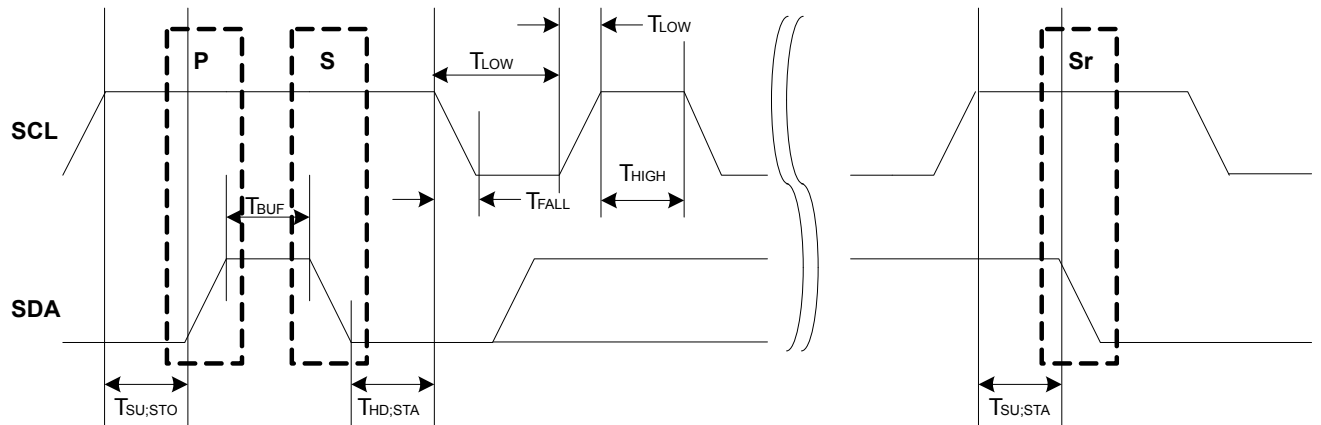
Figure 33-6 SCL Timing
