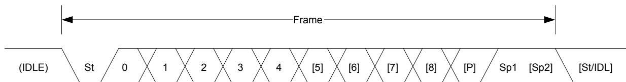
Figure 31-2 Frame Formats
