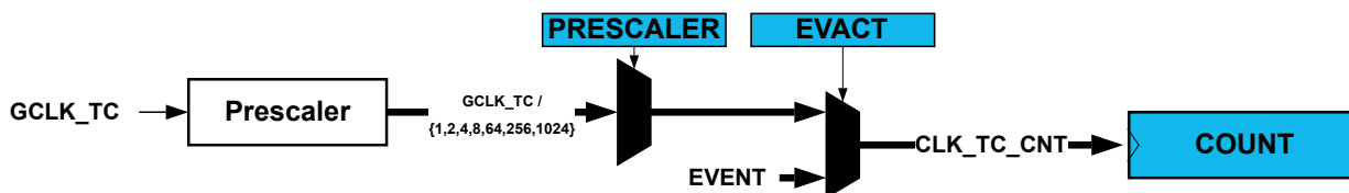
Figure 34-2 Prescaler
