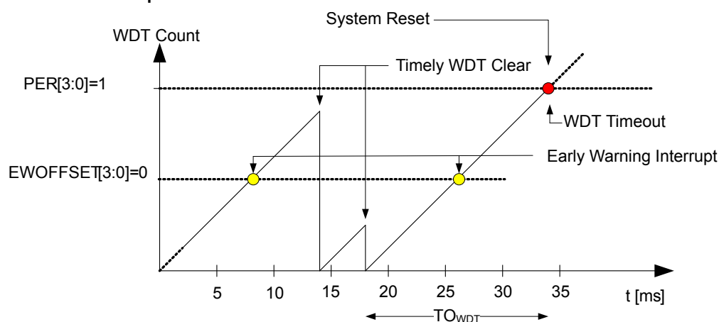
Figure 23-2 Normal-Mode Operation
