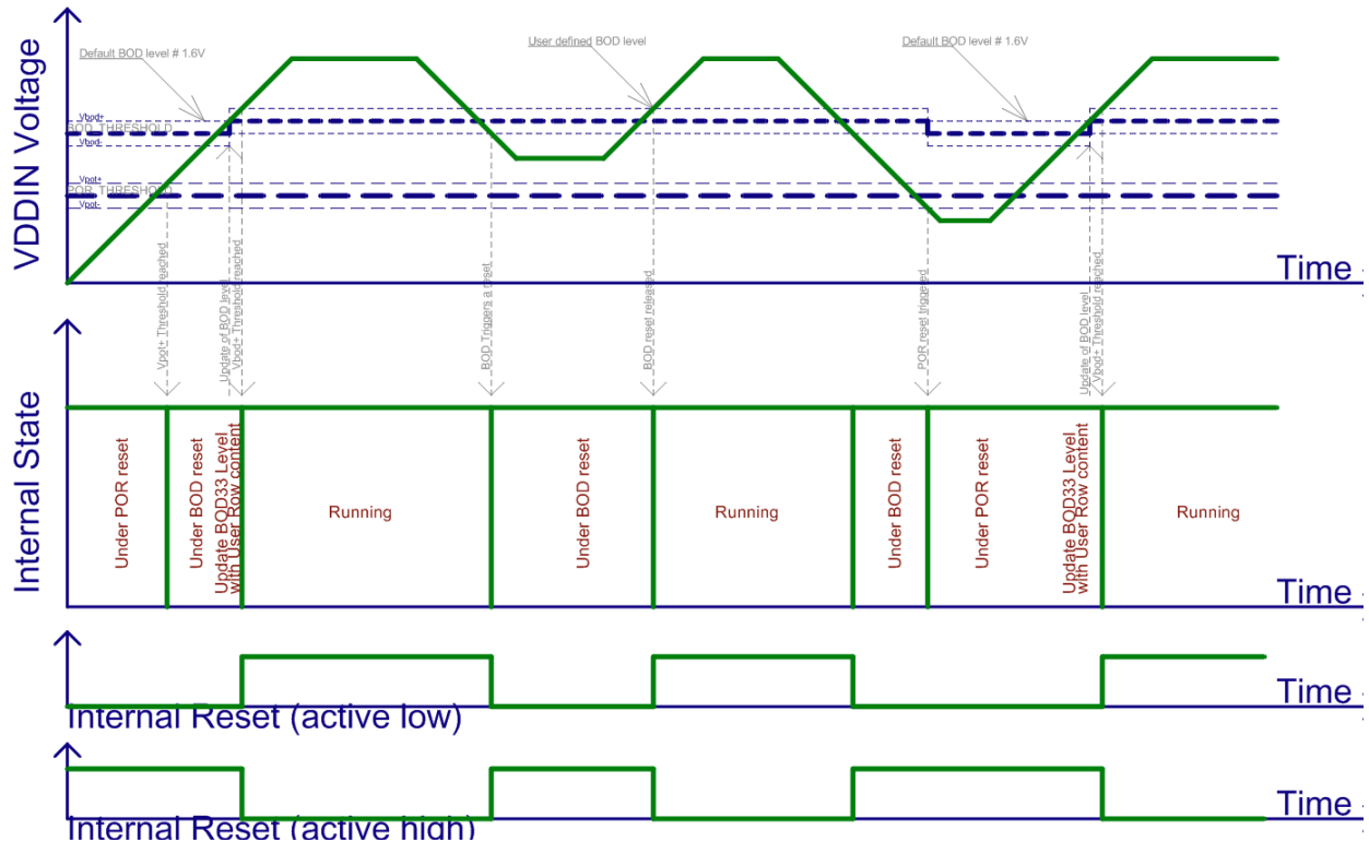
Figure 45-1 POR Operating Principle, Scheme X : BOD reset behave at startup and default levels.
