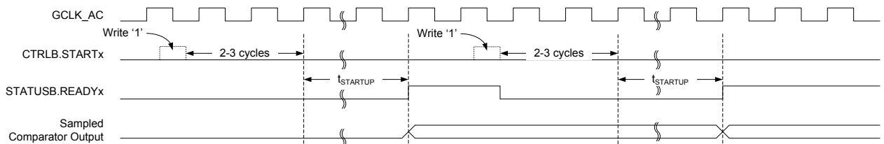
Figure 42-3 Single-Shot Example
