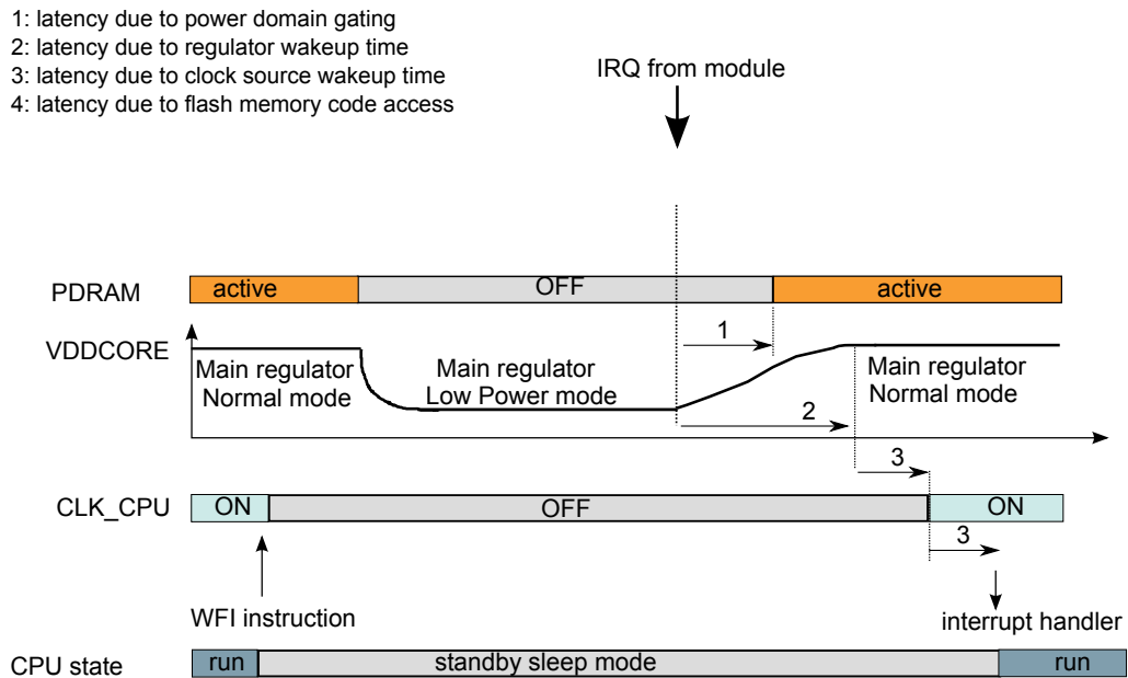
Figure 19-5 Total Wake-up Time from Standby Sleep Mode
