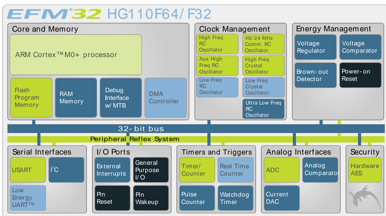
Figure 2.1. Block Diagram
