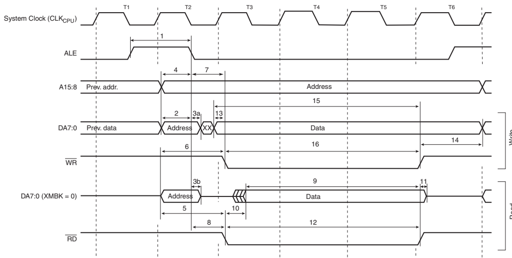
Figure 27-11. External Memory Timing (SRWn1 = 1, SRWn0 = 0)
