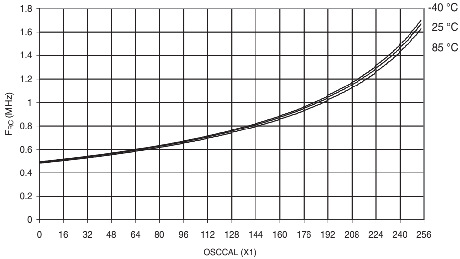
Figure 28-35. 1MHz RC Oscillator Frequency vs. OSCCAL Value
