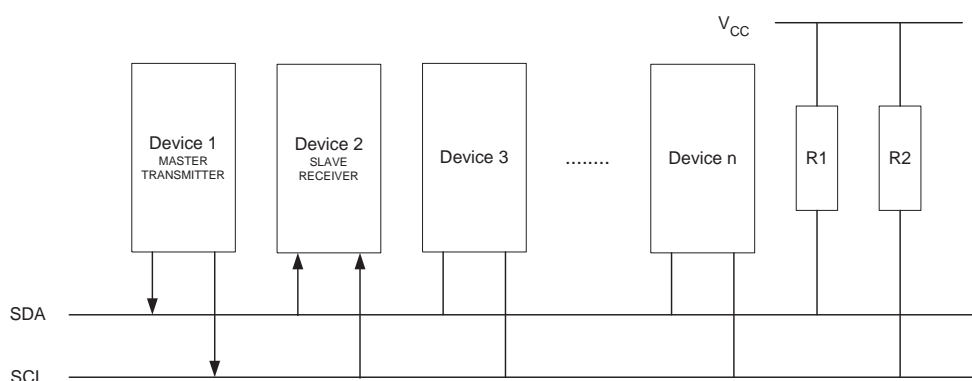
Figure 21-11. Data Transfer in Master Transmitter Mode
