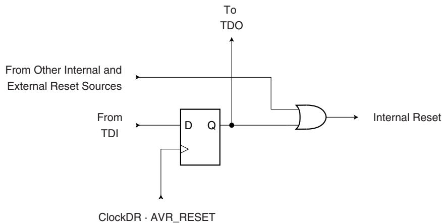
Figure 24-4. Reset Register
