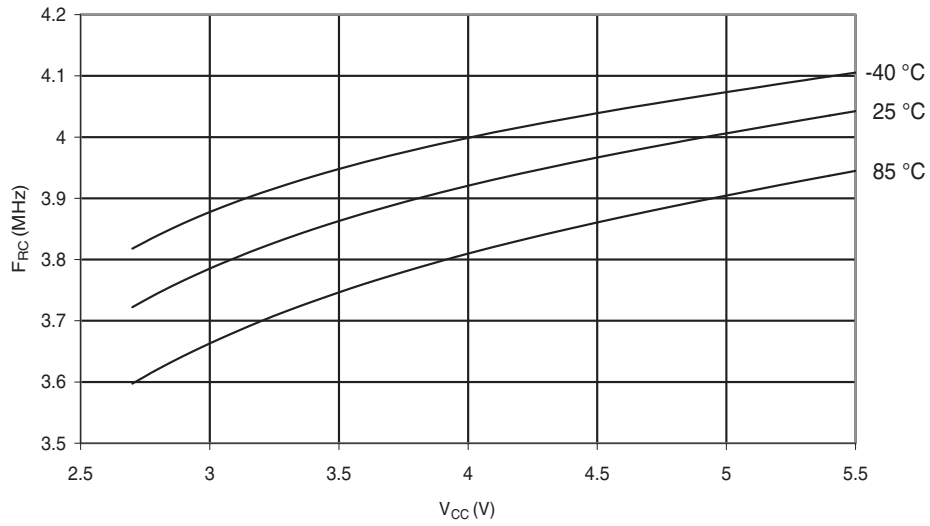
Figure 28-40. Calibrated 4MHz RC Oscillator Frequency vs. V CC
