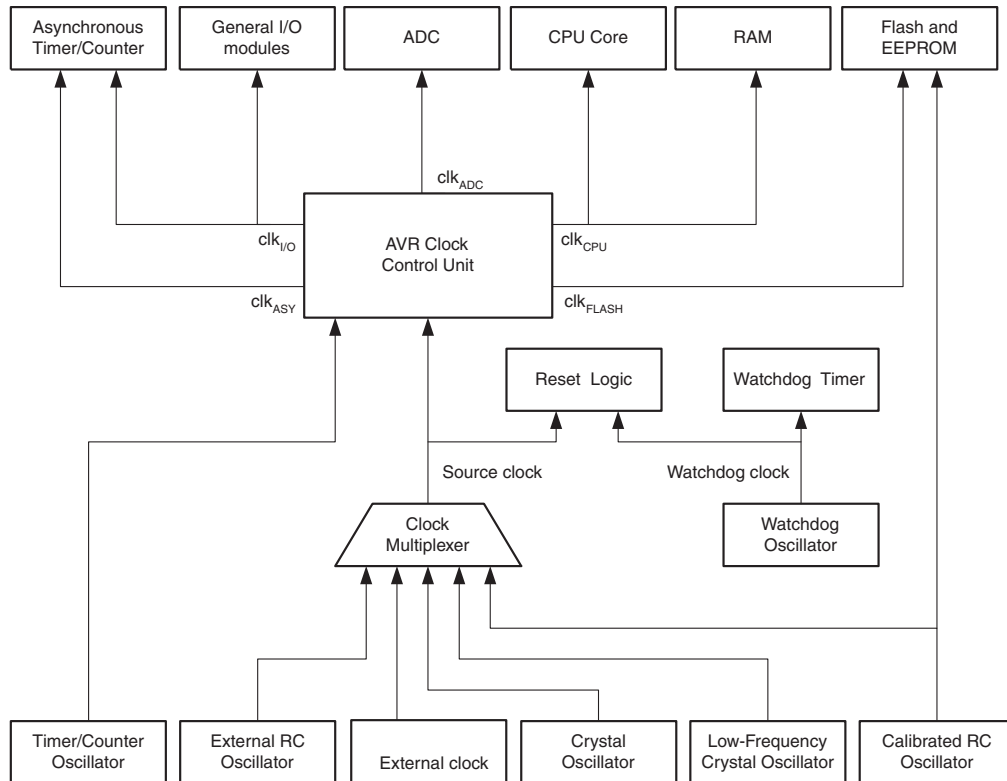
Figure 8-1. Clock Distribution
