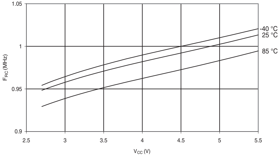
Figure 28-34. Calibrated 1MHz RC Oscillator Frequency vs. V CC
