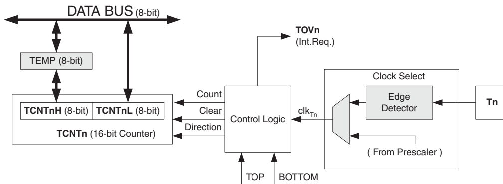
Figure 15-2. Counter Unit Block Diagram
