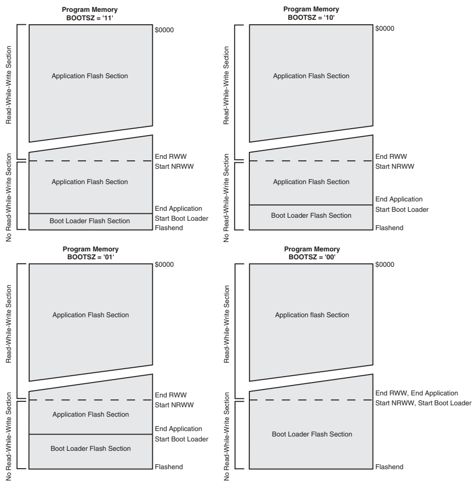
Figure 25-2. Memory Sections (1)
