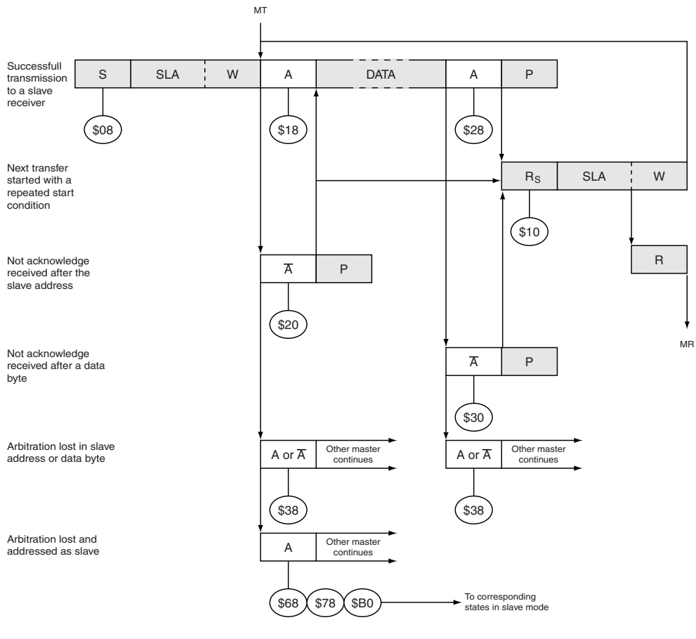
Figure 21-12. Formats and States in the Master Transmitter Mode
