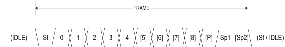
Figure 20-4. Frame Formats
