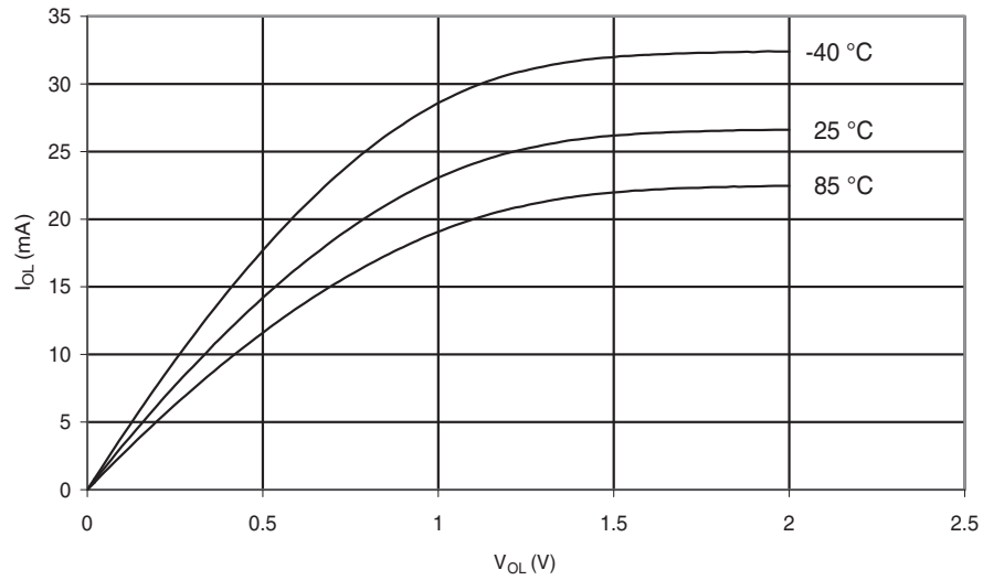
Figure 28-25. I/O Pin Sink Current vs. Output Voltage, V_{CC} = 2.7V
