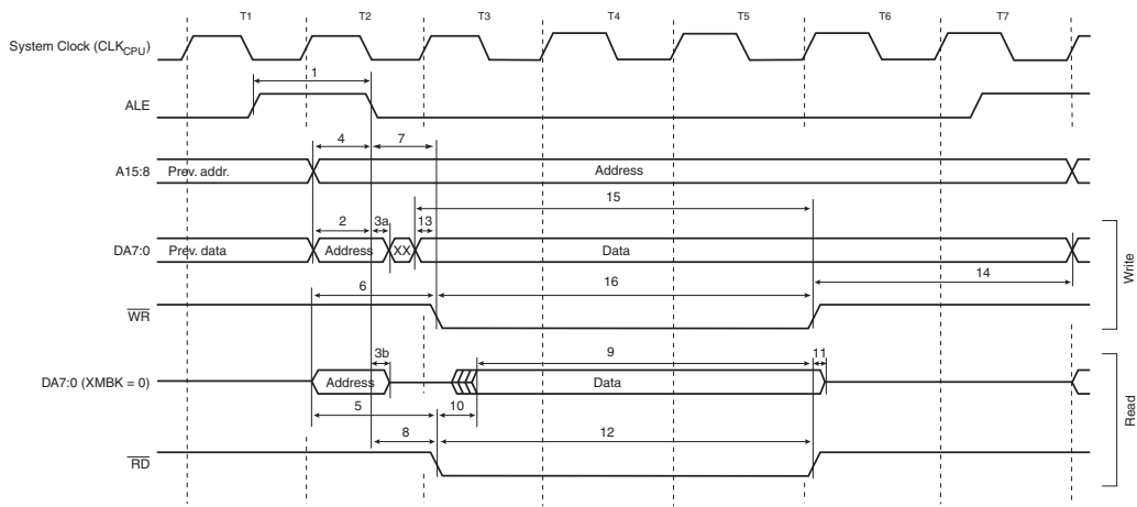
Figure 27-12. External Memory Timing (SRWn1 = 1, SRWn0 = 1) 0
