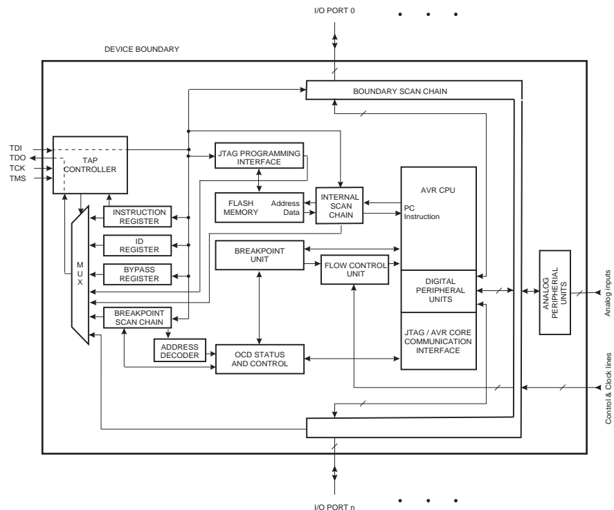
Figure 24-1. Block Diagram
