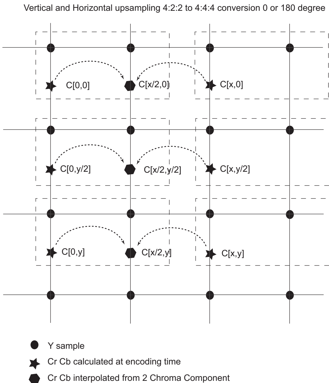
Figure 33-2. 4:2:2 Upsampling Algorithm
