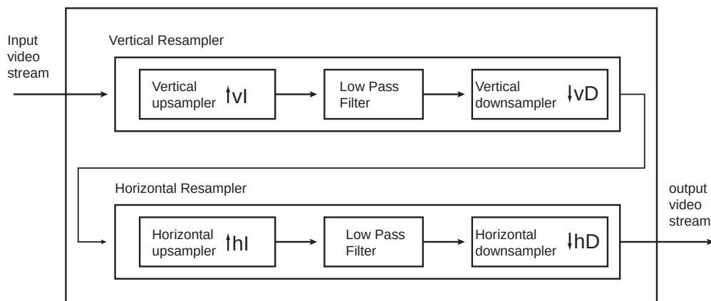
Figure 33-6. Video Resampler Architecture
