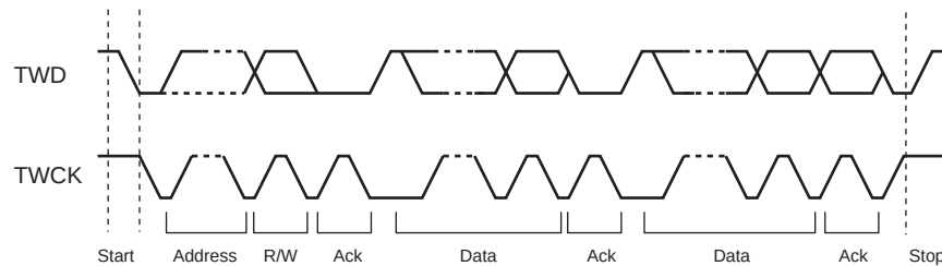
Figure 41-3. Transfer Format
