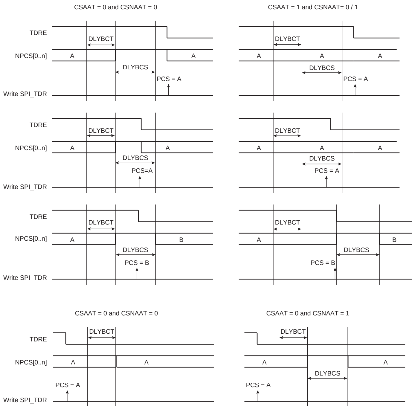
Figure 40-11. Peripheral Deselection
