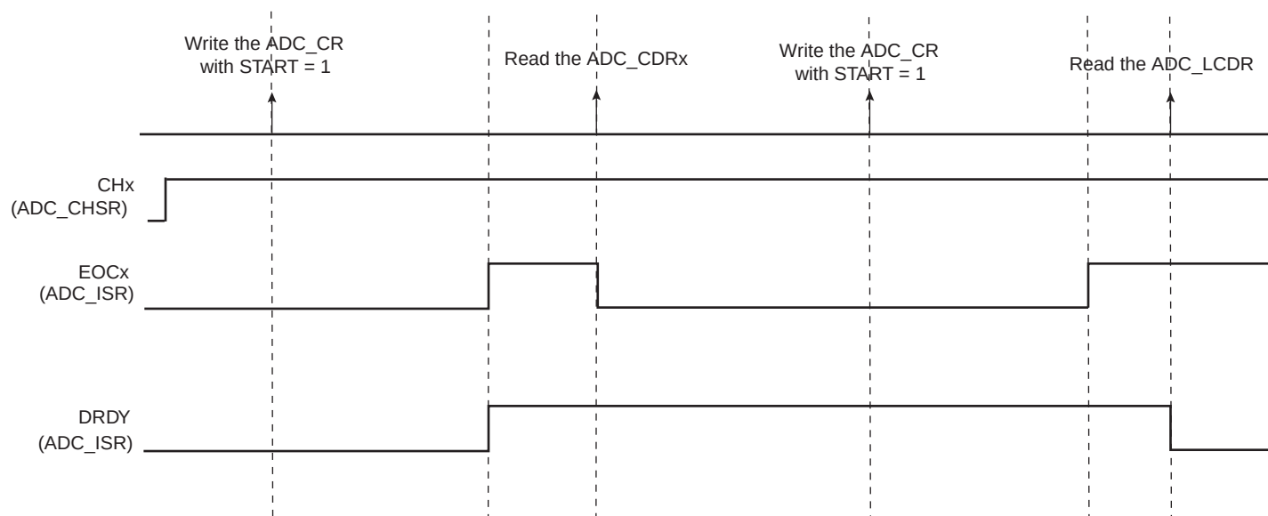
Figure 50-4. EOCx and DRDY Flag Behavior
