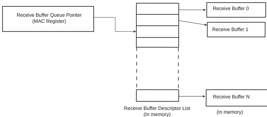
Figure 38-2. Receive Buffer List
