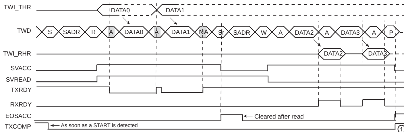
Figure 41-30. Repeated Start + Reversal from Read to Write Mode
