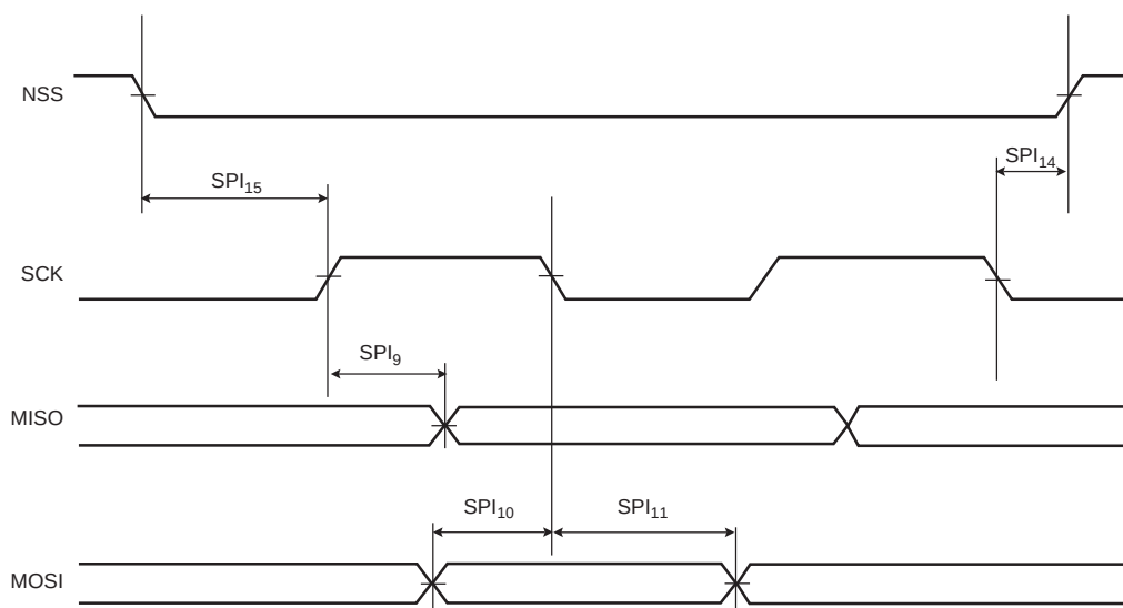
Figure 55-34. USART SPI Slave Mode (Mode 0 or 3)
