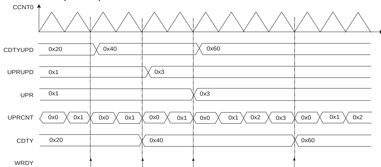
Figure 49-11. Method 2 (UPDM = 1)
