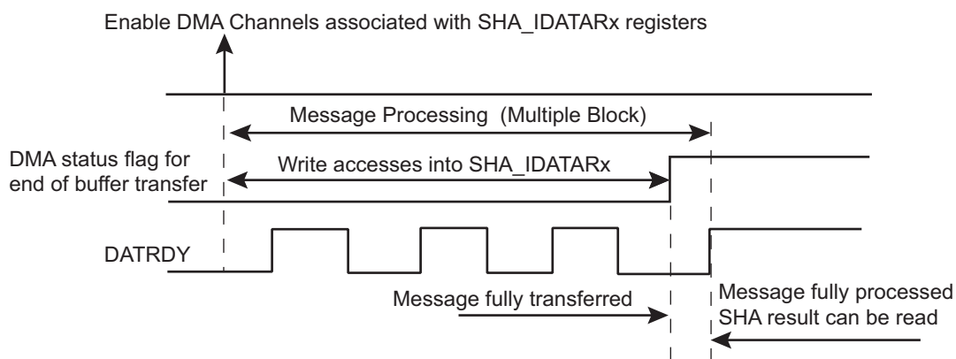
Figure 54-1. interrupts Processing with DMA
