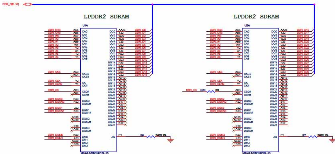
Figure 29-4. 2x16-bit LPDDR2 Hardware Configuration
