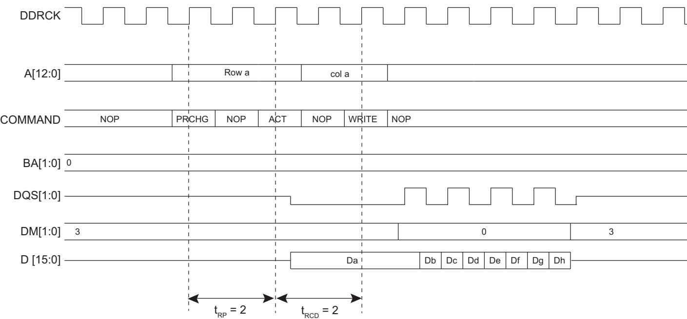
Figure 30-4. Burst Write Access, Row Closed, DDR-SDRAM Devices
