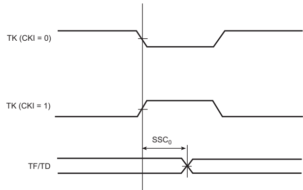
Figure 55-19. SSC Transmitter, TK and TF as Output
