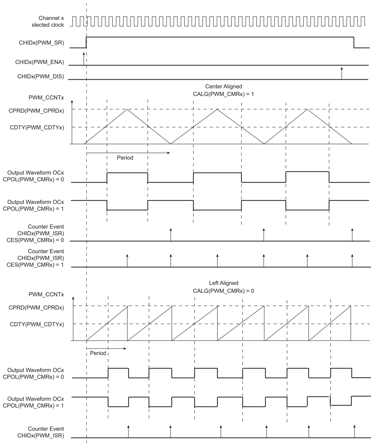
Figure 49-5. Waveform Properties
