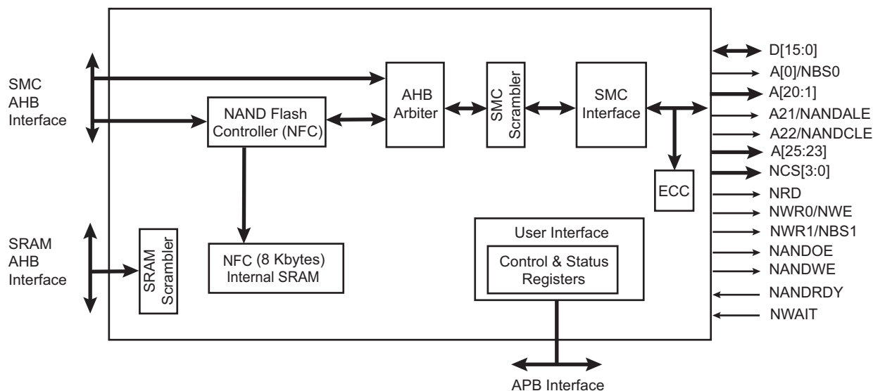
Figure 31-1. Block Diagram
