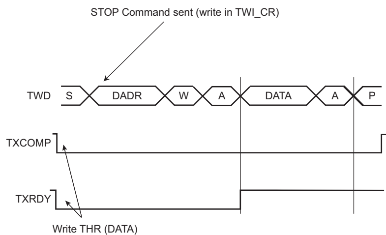
Figure 41-5. Master Write with One Data Byte
