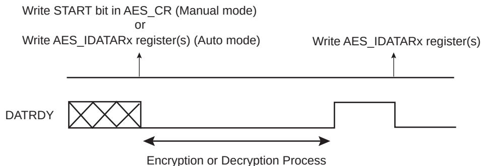
Figure 52-2. Manual and Auto Modes with AES_MR.LOD = 1
