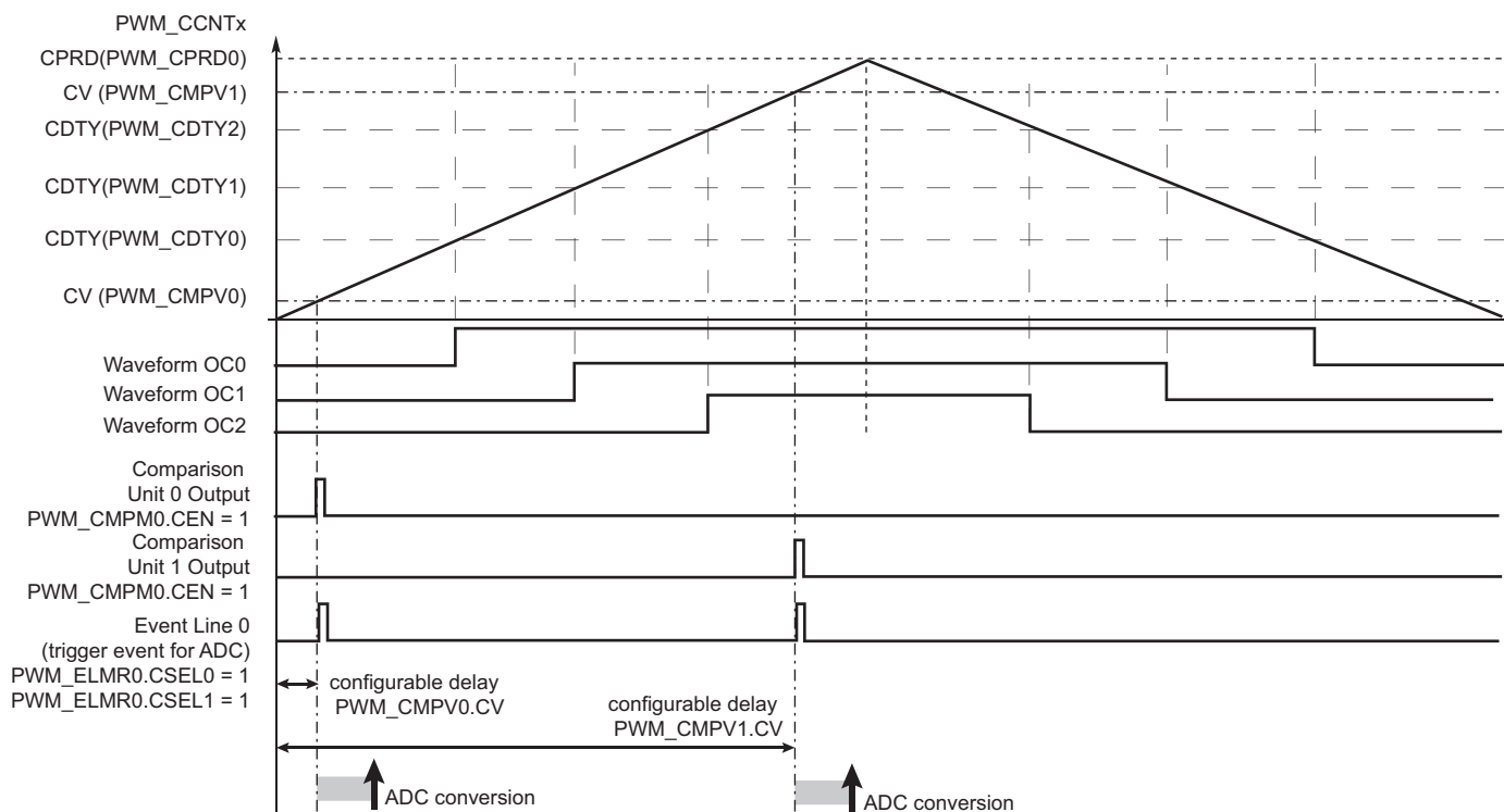
Figure 49-15. Event Line Generation Waveform (Example)
