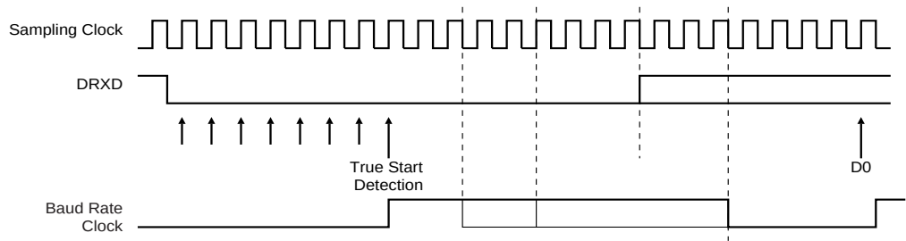
Figure 43-4. Start Bit Detection
