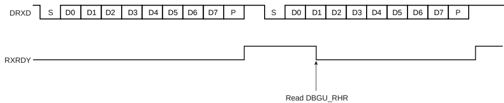
Figure 43-6. Receiver Ready
