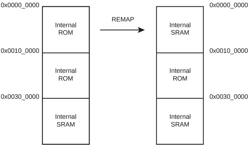
Figure 12-4. Remap Action after Download Completion
