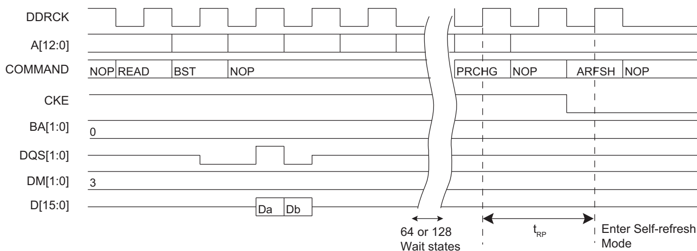
Figure 30-14. Self-refresh Mode Entry, Time-out = 1 or 2
