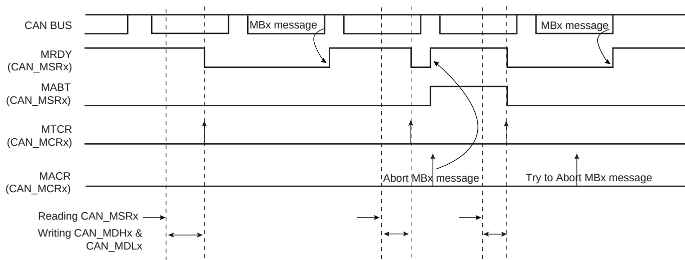
Figure 46-15. Transmitting Messages
