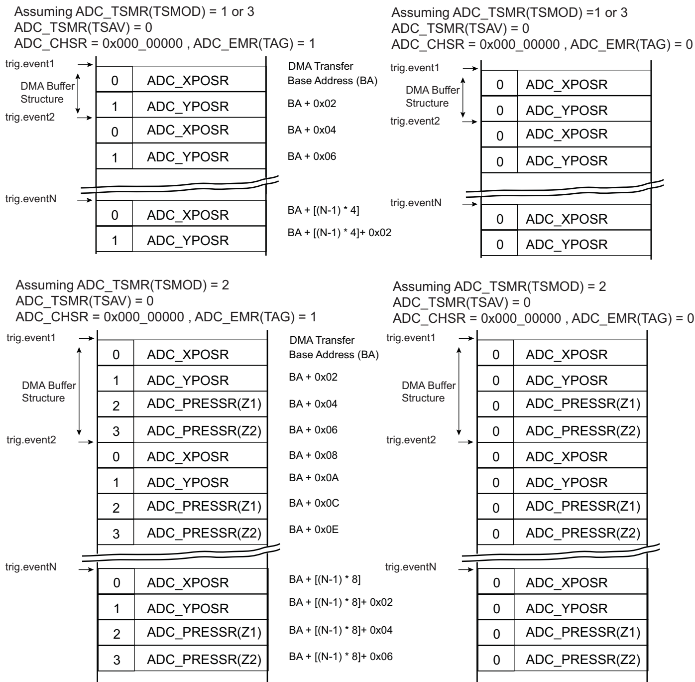
Figure 50-16. Buffer Structure When Only Touchscreen Channels are Enabled
