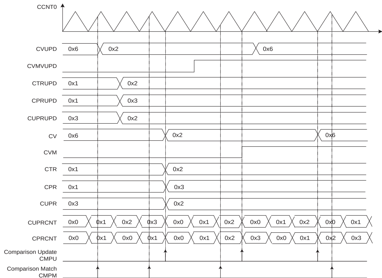
Figure 49-13. Comparison Waveform
