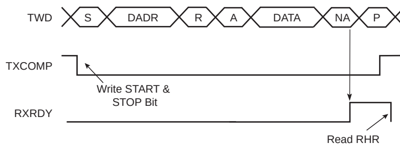
Figure 41-8. Master Read with One Data Byte
