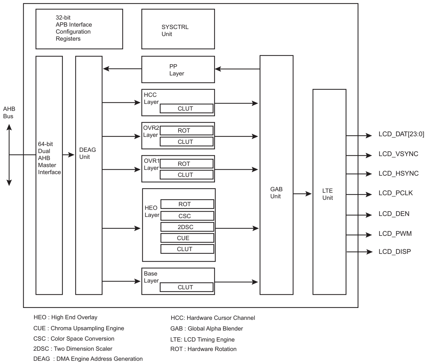
Figure 33-1. Block Diagram
