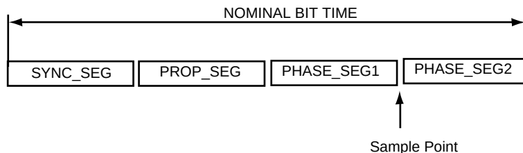
Figure 46-4. Partition of the CAN Bit Time
