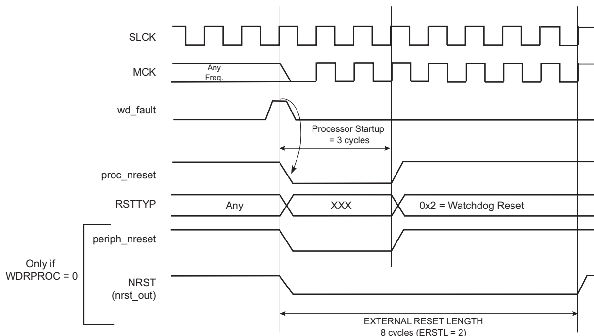
Figure 19-8. Watchdog Reset
