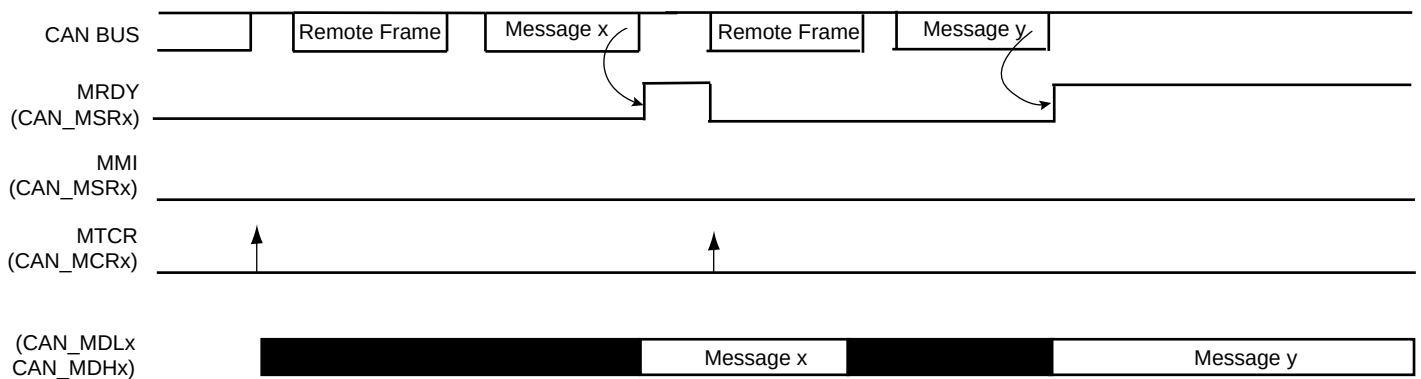
Figure 46-18. Consumer Handling
