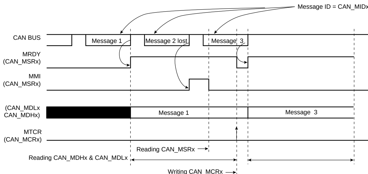
Figure 46-11. Receive Mailbox
