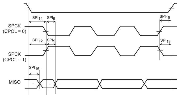
Figure 55-16. SPI Slave Mode - NPCS Timings
