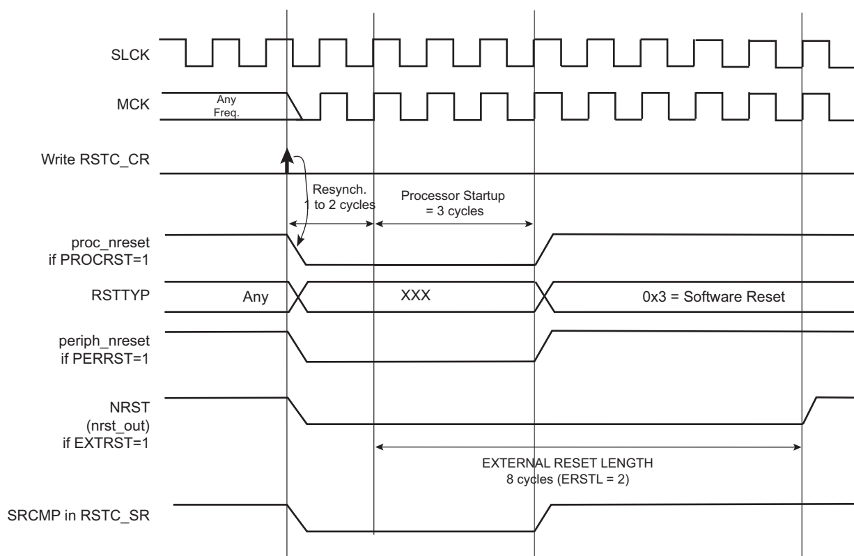
Figure 19-7. Software Reset
