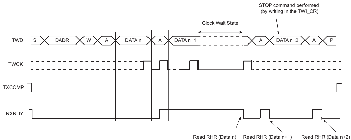
Figure 41-10. Master Read Wait State with Multiple Data Bytes
