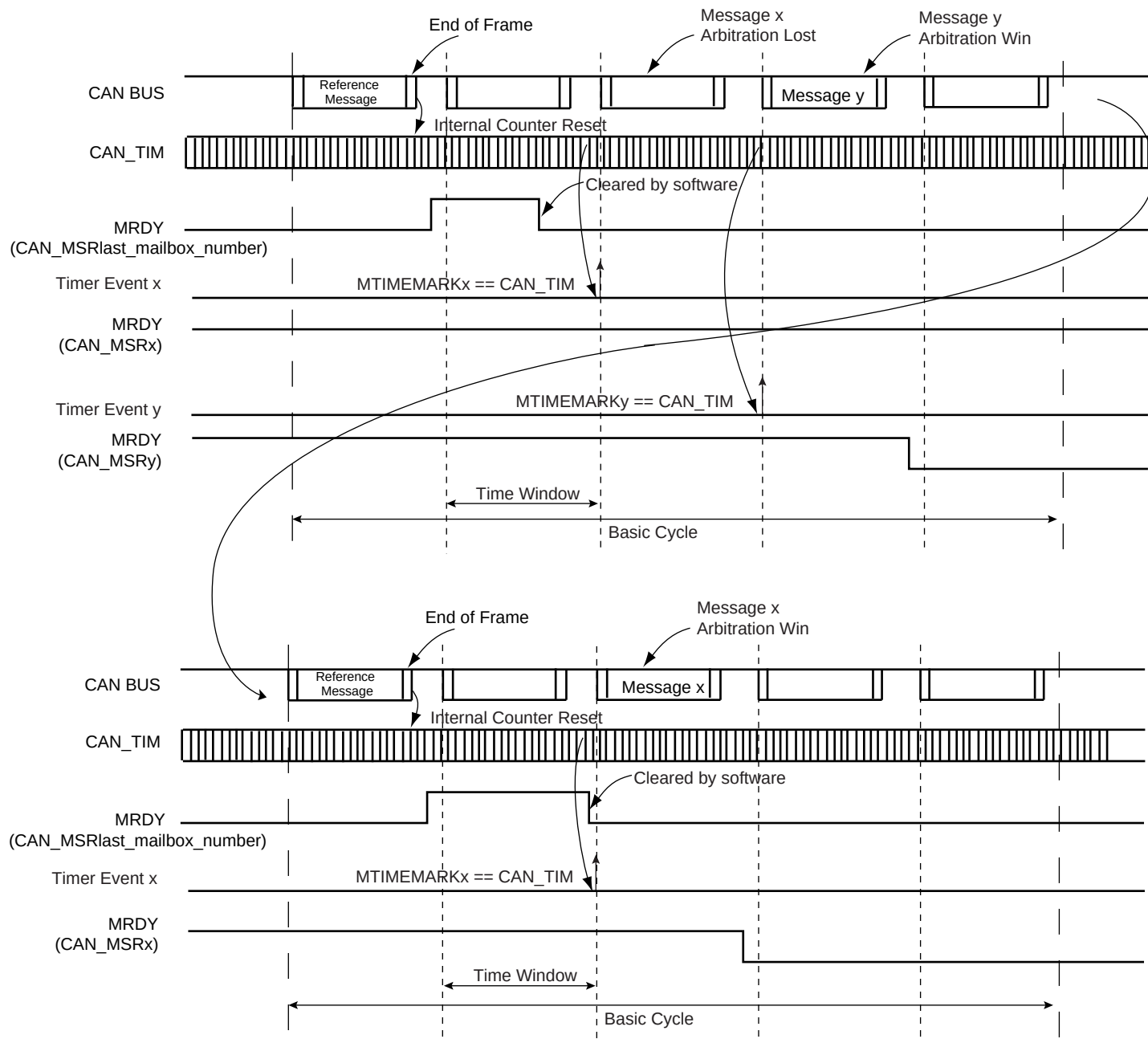
Figure 46-21. Time Triggered Operations
