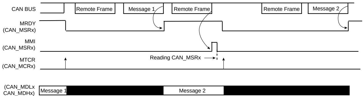
Figure 46-17. Producer Handling
