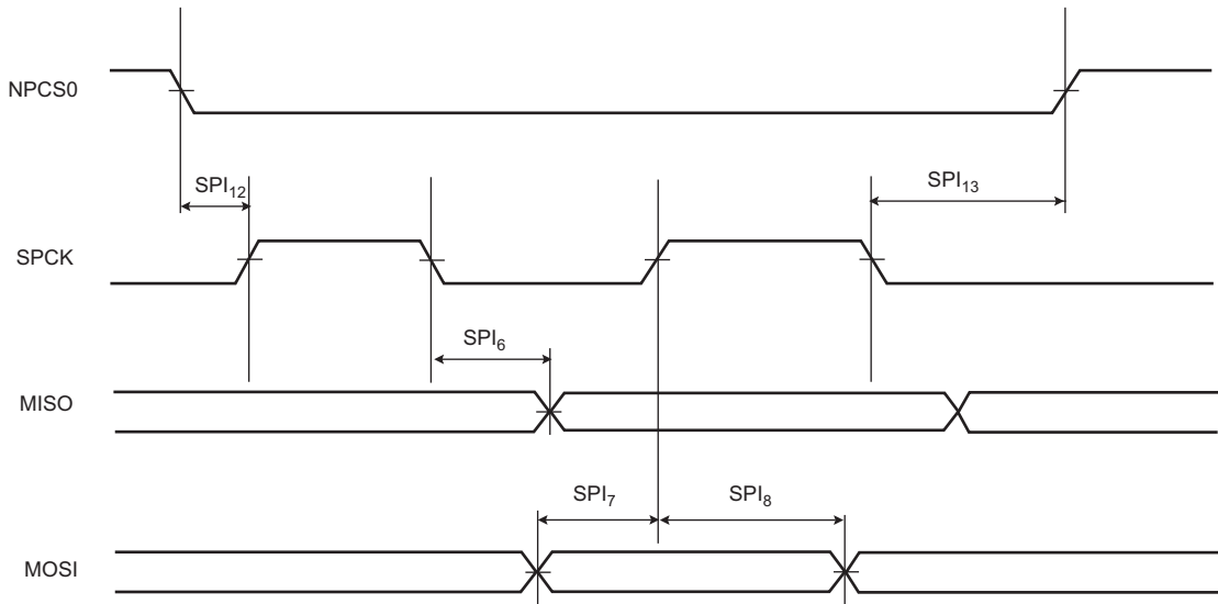
Figure 55-33. USART SPI Slave Mode (Mode 1 or 2)
