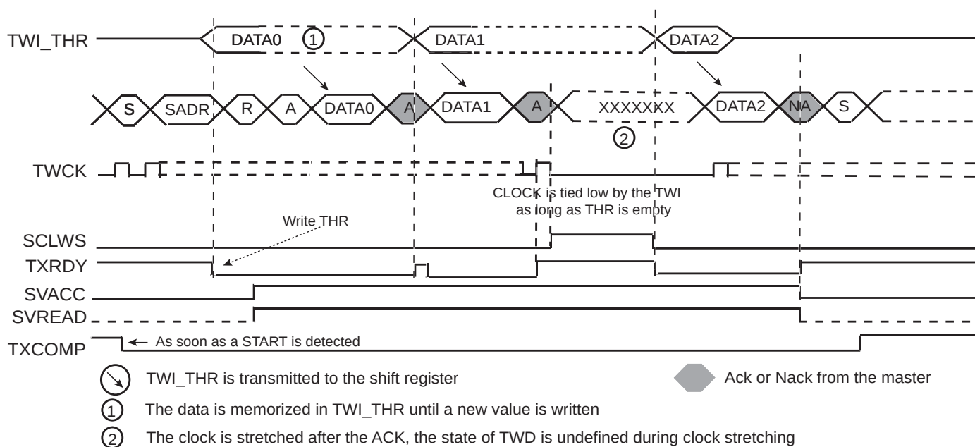
Figure 41-28. Clock Stretching in Read Mode
