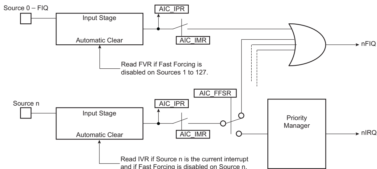
Figure 17-10. Fast Forcing
