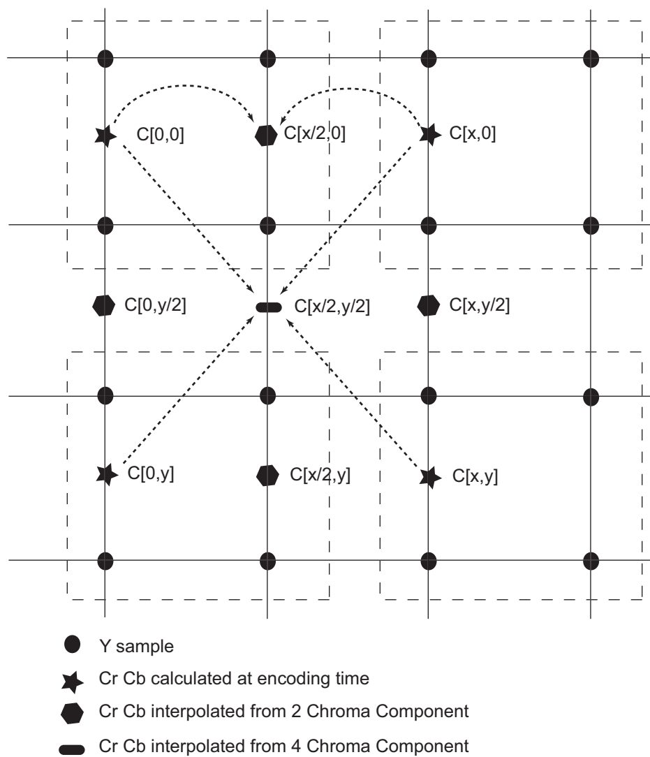
Figure 33-5. 4:2:0 Upsampling Algorithm
