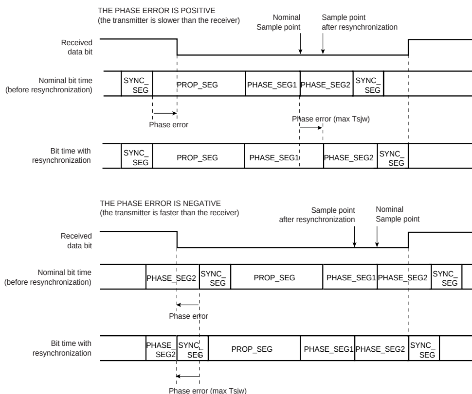
Figure 46-6. CAN Resynchronization
