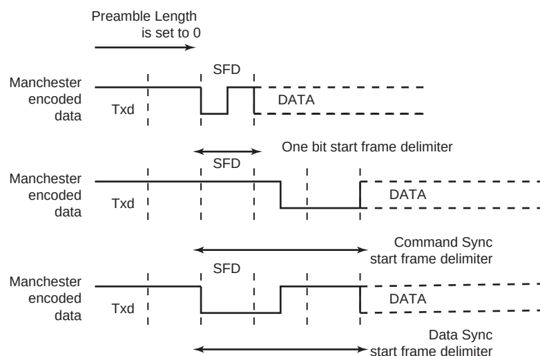
Figure 45-9. Start Frame Delimiter
