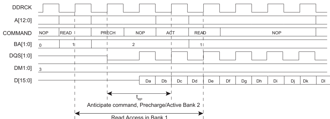
Figure 30-19. Anticipate Precharge/Activate Command in Bank 2 during Read Access in Bank 1
