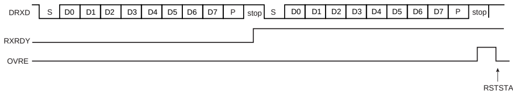
Figure 43-7. Receiver Overrun
