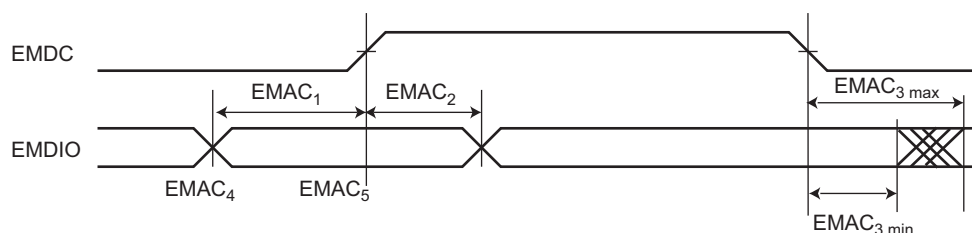
Figure 55-29. Min and Max Access Time of EMAC Output Signals
