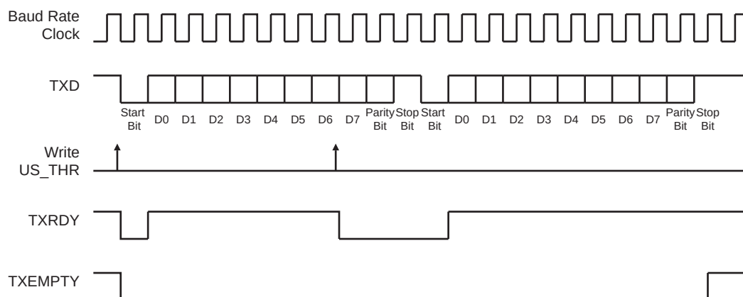
Figure 45-6. Transmitter Status
