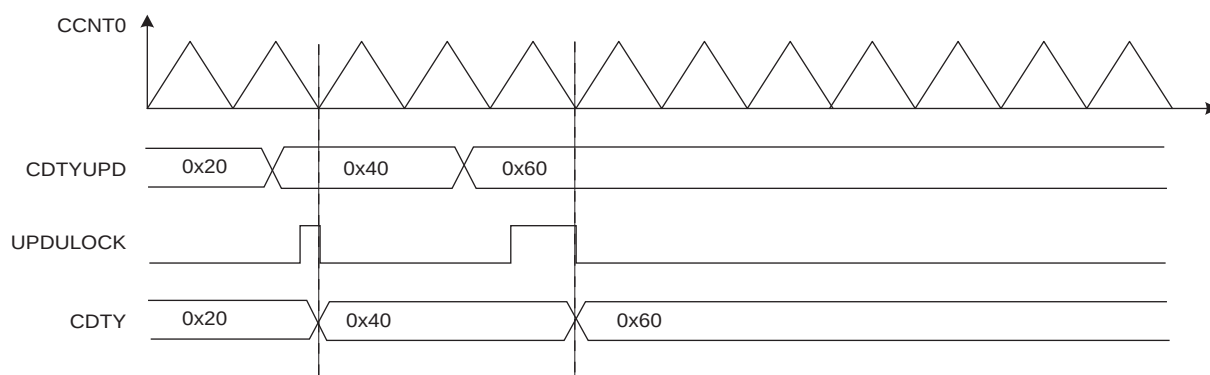
Figure 49-10. Method 1 (UPDM = 0)
