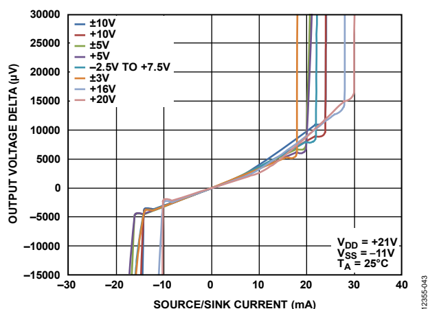
Figure 45. Source and Sink Capability of Output Amplifier with Positive Full Scale Loaded
