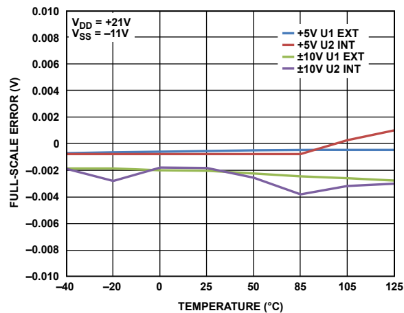
Figure 23. Full-Scale Error vs. Temperature
