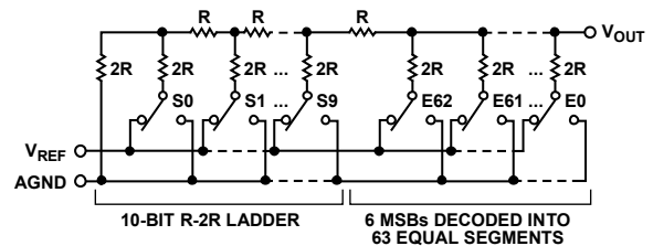
Figure 73. DAC Ladder Structure
