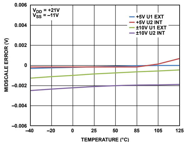
Figure 22. Midscale Error vs. Temperature
