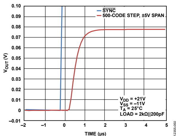
Figure 52. 500-Code Step Settling Time, \pm 5 V Range
