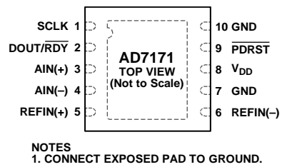
Figure 5. Pin Configuration
