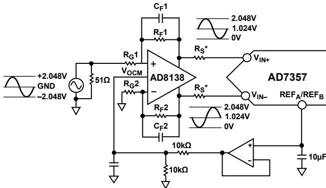
*MOUNT AS CLOSE TO THE AD7357 AS POSSIBLE AND ENSURE THAT HIGH PRECISION R_S RESISTORS ARE USED. R_S = 33\Omega ; R_{G1} = R_{F1} = R_{F2} = 499\Omega ; C_{F1} = C_{F2} = 39pF ; R_{G2} = 523\Omega
