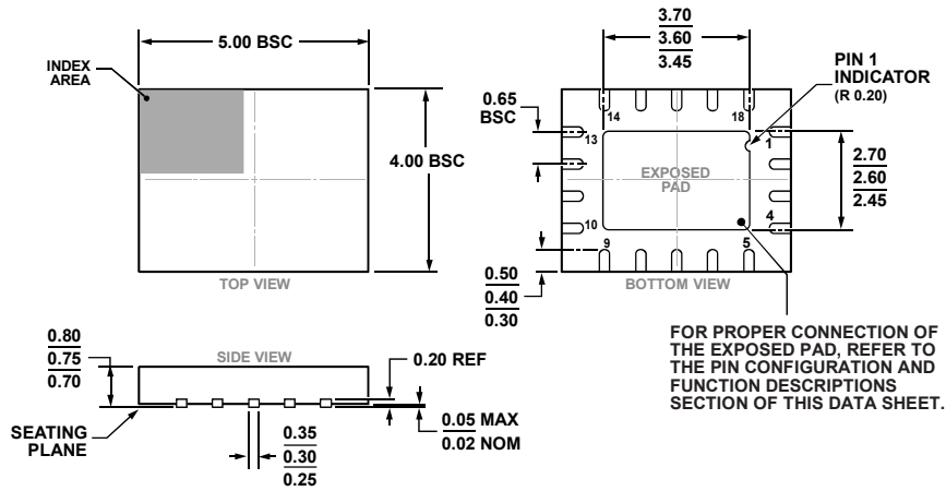
Figure 343. 18-Lead Lead Frame Chip Scale Package [LFCSP_WQ] 5mm x 4 mm Body, Very Very Thin Quad (CP-18-1) Dimensions shown in millimeters
