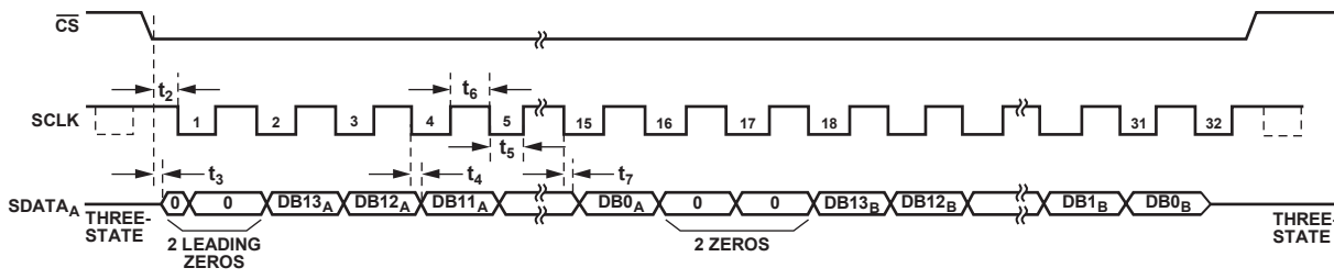
Figure 32. Reading Data from Both ADCs on One SDATA Line with 32 SCLKs
