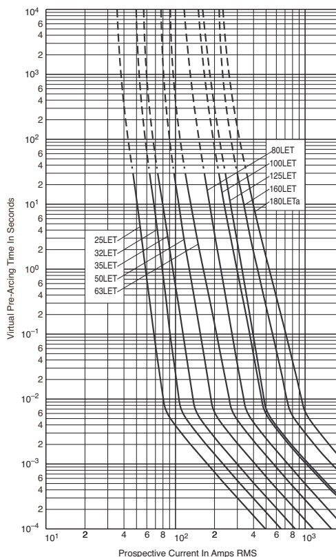
Time-Current Curve
