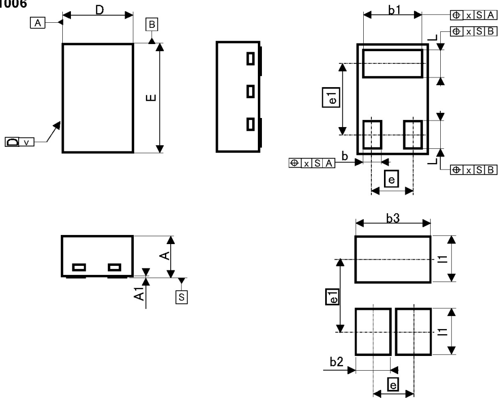
Pattern of terminal position areas [Not a recommended pattern of soldering pad]
