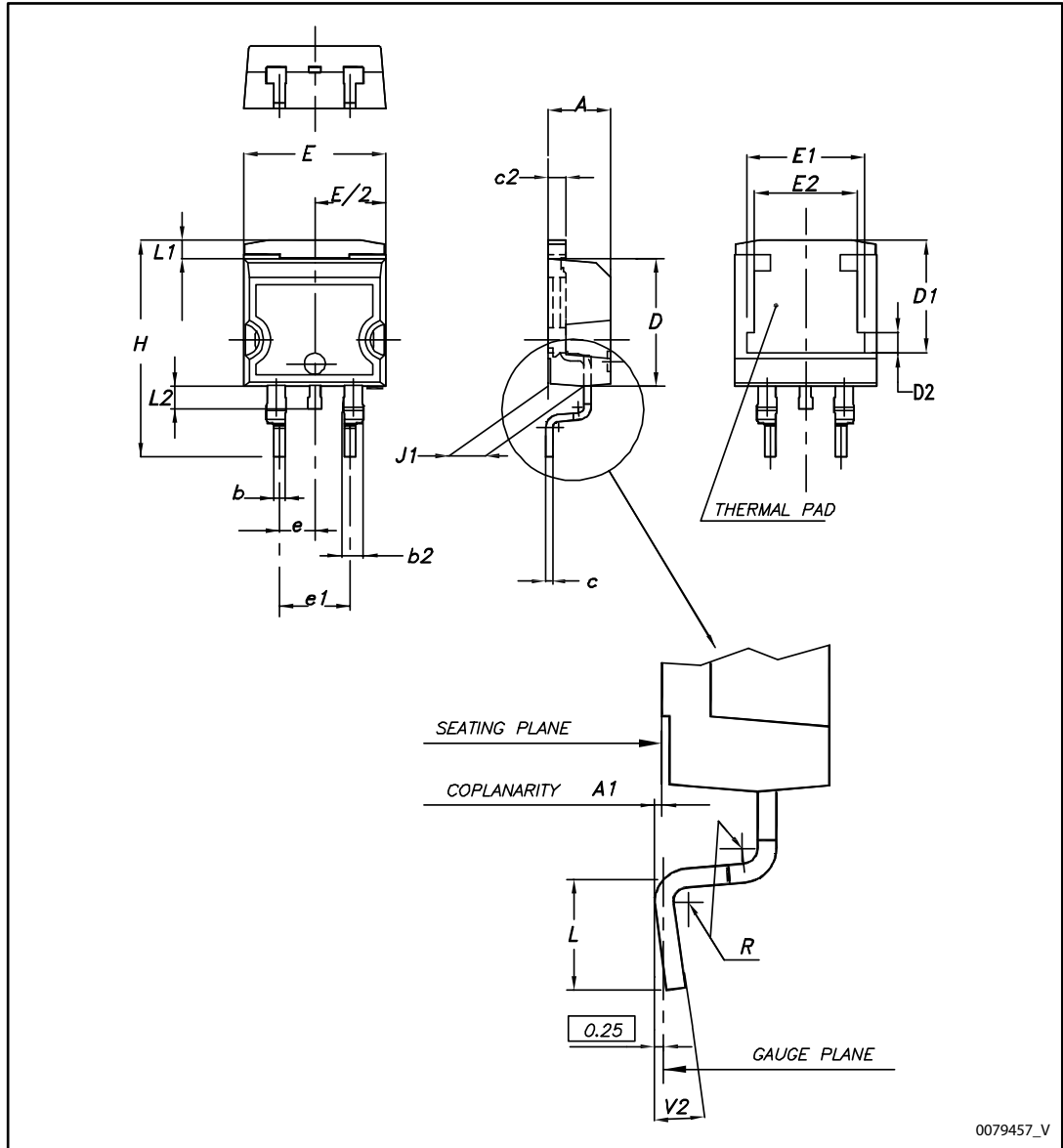
Figure 33: D 2 PAK (TO-263) type A package outline
