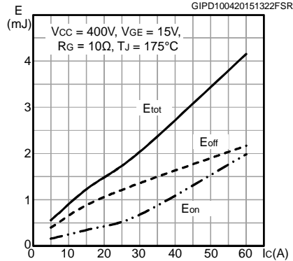
Figure 16: Switching loss vs. collector current
