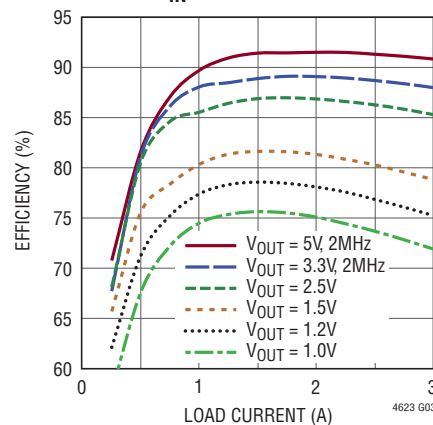
Efficiency vs Load Current with 16V IN
