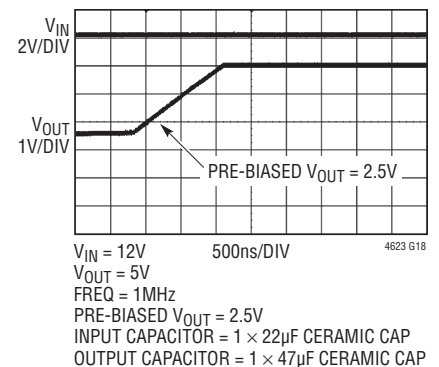
Start into Pre-Biased Output
