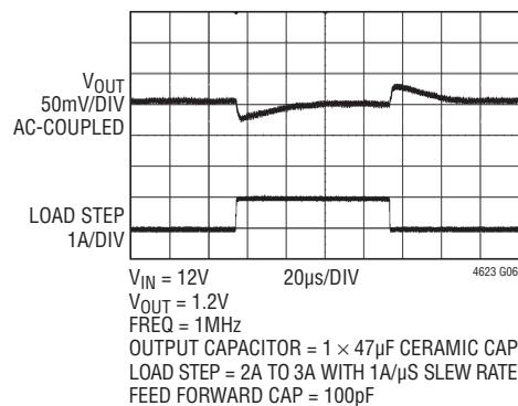
1.2V Output Transient Response
