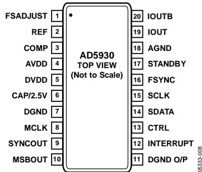
Figure 8. Pin Configuration
