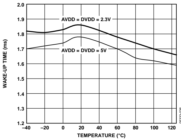
Figure 17. Wake-up Time vs. Temperature
