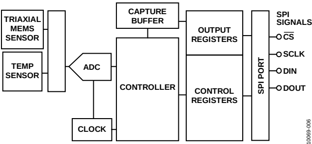
Figure 6. Simplified Sensor Signal Processing Block Diagram
