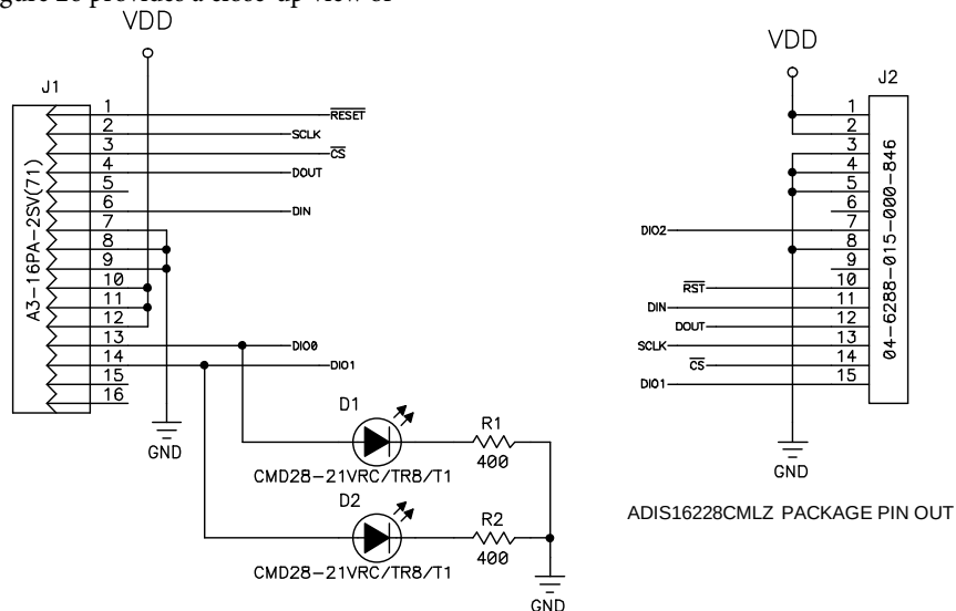
Figure 27. Electrical Schematic
