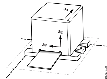
Figure 19. Accelerometer Axial and Polarity Definitions
