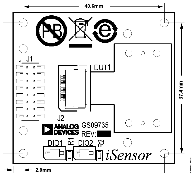
Figure 25. PCB Assembly View and Dimensions
