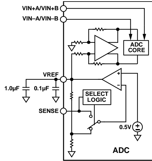
Figure 48. Internal Reference Configuration
