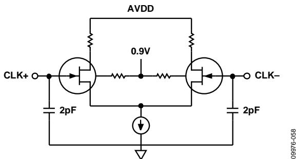
Figure 51. Equivalent Clock Input Circuit
