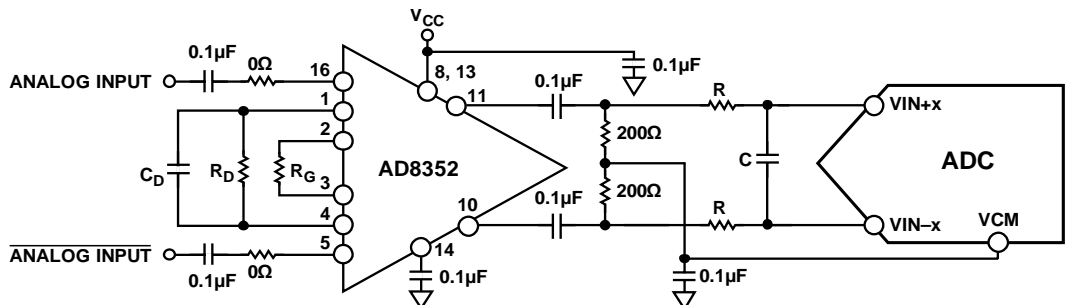
Figure 47. Differential Input Configuration Using the AD8352
