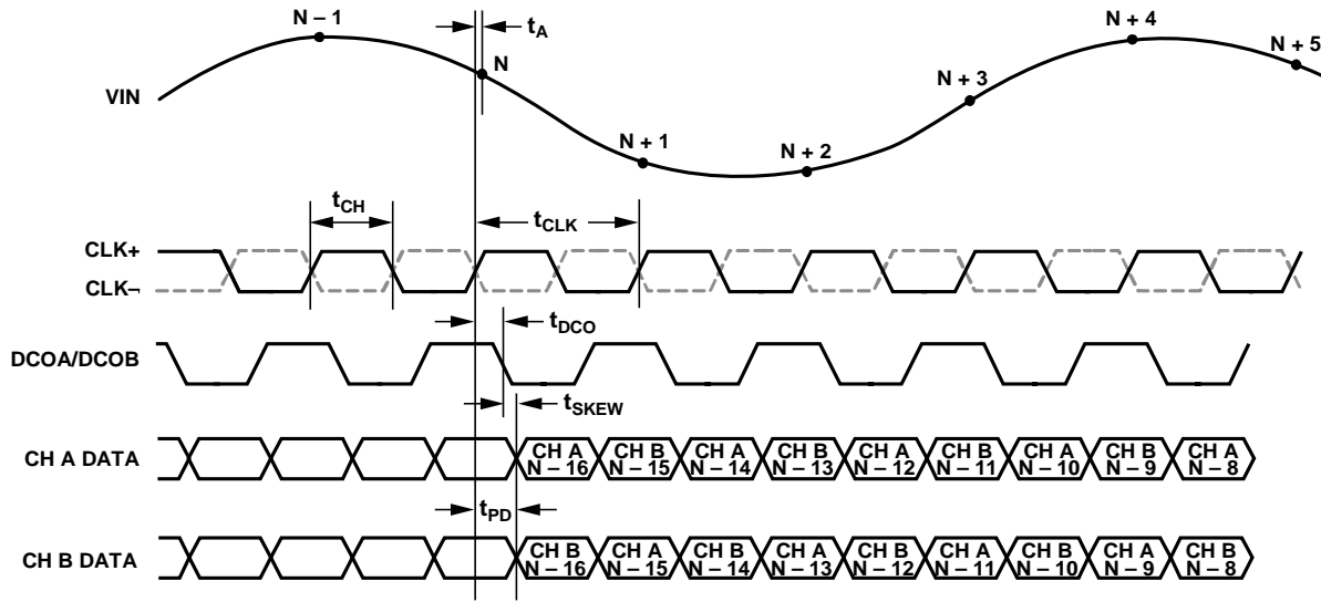
Figure 3. CMOS Interleaved Output Mode Data Output Timing
