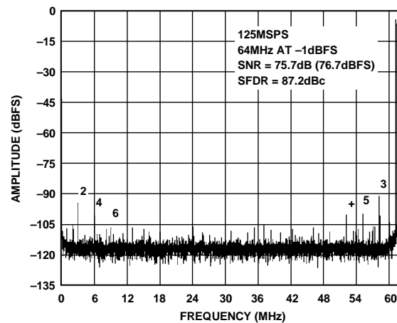
Figure 9. Single-Tone 16k FFT with f_{IN} = 64 MHz , f_{SAMPLE} = 125 MSPS , V_{REF} = 1.0 V
