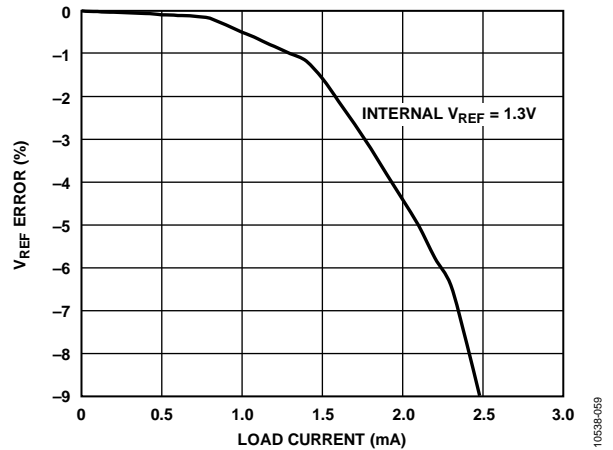
Figure 59. V_{REF} = 1.3V Error vs. Load Current
