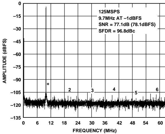
Figure 7. Single-Tone 16k FFT with f_{IN} = 9.7 MHz , f_{SAMPLE} = 125 MSPS , V_{REF} = 1.0 V
