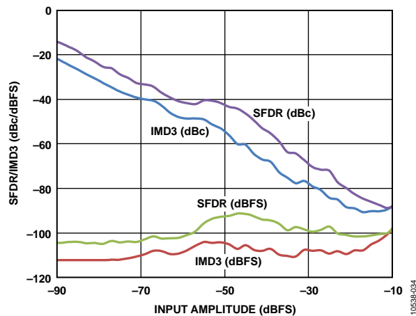
Figure 34. Two-Tone SFDR/IMD3 vs. Input Amplitude ( A_{IN} ) with f_{IN1} = 70.5 MHz and f_{IN2} = 72.5 MHz, f_{SAMPLE} = 125 MSPS, V_{REF} = 1.3 V
