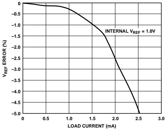
Figure 58. V_{REF} = 1.0V Error vs. Load Current
