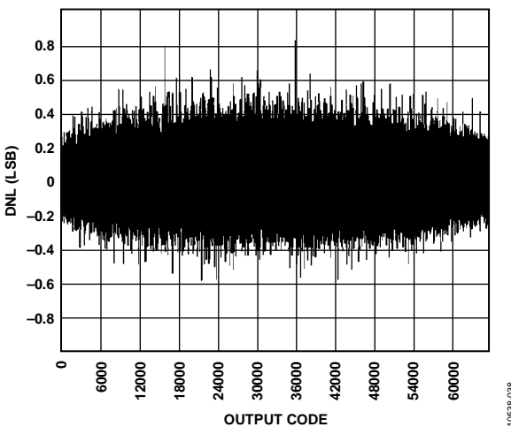
Figure 38. DNL, f_{IN} = 9.7 MHz, f_{SAMPLE} = 125 MSPS, V_{REF} = 1.3 V
