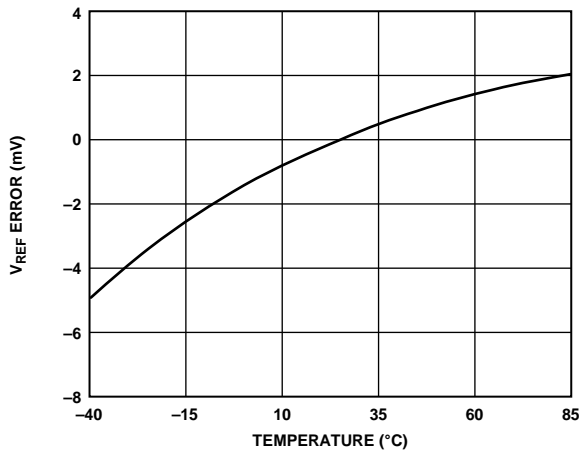
Figure 60. Typical V_{REF} = 1.0 V Drift
