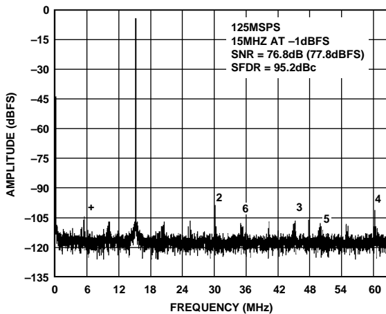
Figure 8. Single-Tone 16k FFT with f_{IN} = 15 MHz , f_{SAMPLE} = 125 MSPS , V_{REF} = 1.0 V
