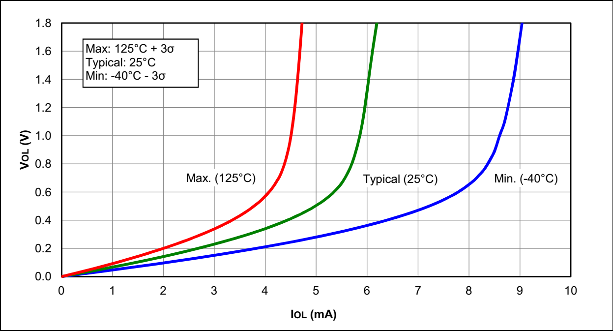
FIGURE 37-6: V_{OL} vs. I_{OL} OVER TEMPERATURE, V_{DD} = 1.8V , PIC16LF1773/6 ONLY
