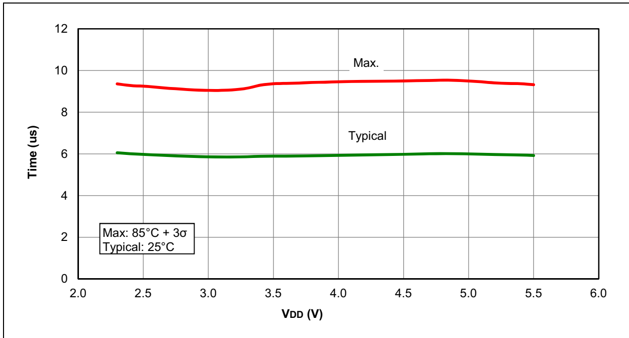
FIGURE 37-24: SLEEP MODE, WAKE PERIOD WITH HFINTOSC SOURCE, VREGPM = 0, PIC16F1773/6 ONLY
