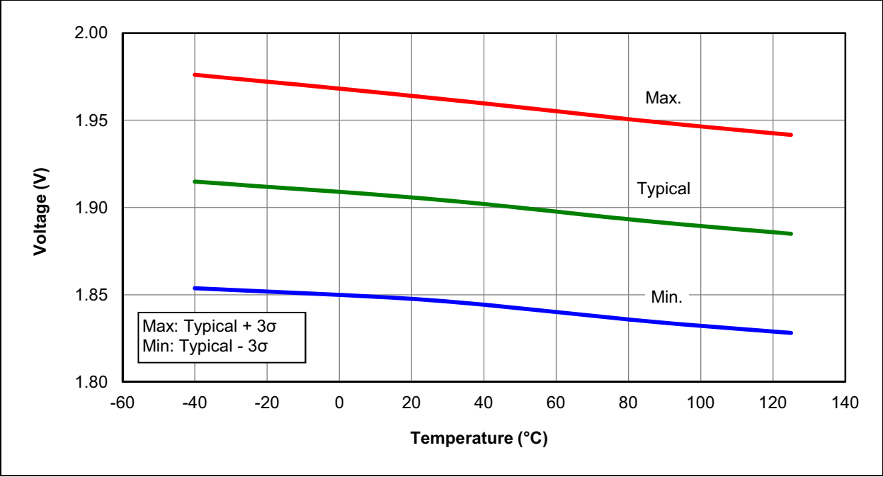
FIGURE 37-9: BROWN-OUT RESET VOLTAGE, BORV = 1, PIC16LF1773/6 ONLY
