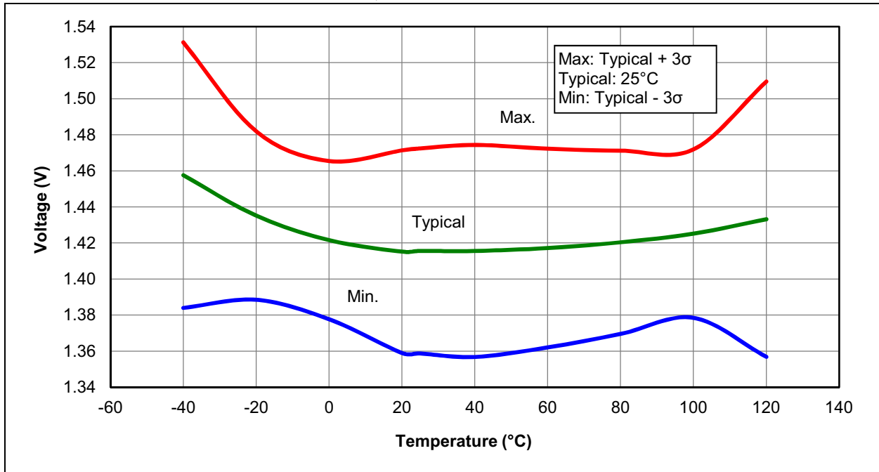
FIGURE 37-8: POR REARM VOLTAGE, PIC16F1773/6 ONLY
