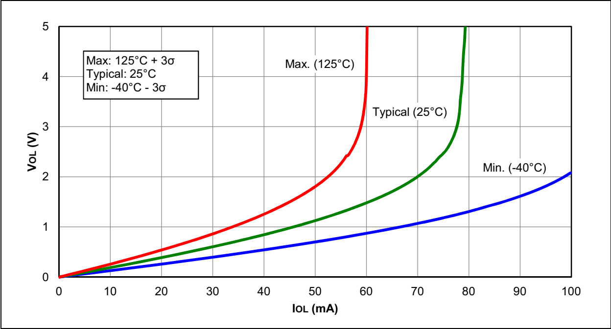
FIGURE 37-2: V_{OL} vs. I_{OL} OVER TEMPERATURE, V_{DD} = 5.5V , PIC16F1773/6 ONLY
