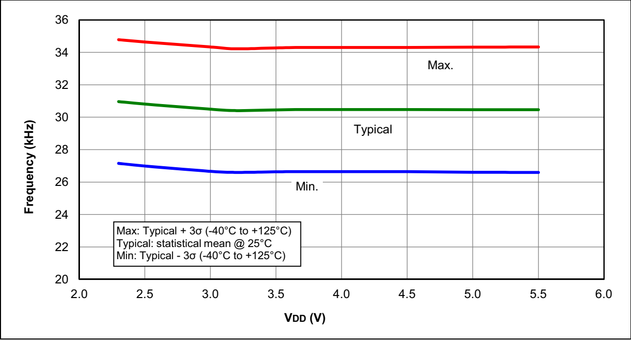
FIGURE 37-21: LFINTOSC FREQUENCY OVER VDD AND TEMPERATURE, PIC16F1773/6 ONLY
