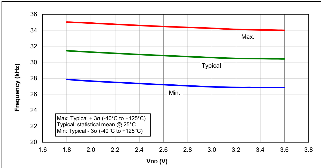
FIGURE 37-20: LFINTOSC FREQUENCY OVER VDD AND TEMPERATURE, PIC16LF1773/6 ONLY
