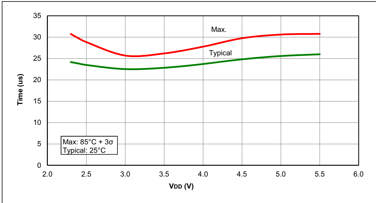
FIGURE 37-23: LOW-POWER SLEEP MODE, WAKE PERIOD WITH HFINTOSC SOURCE, VREGPM = 1, PIC16F1773/6 ONLY
