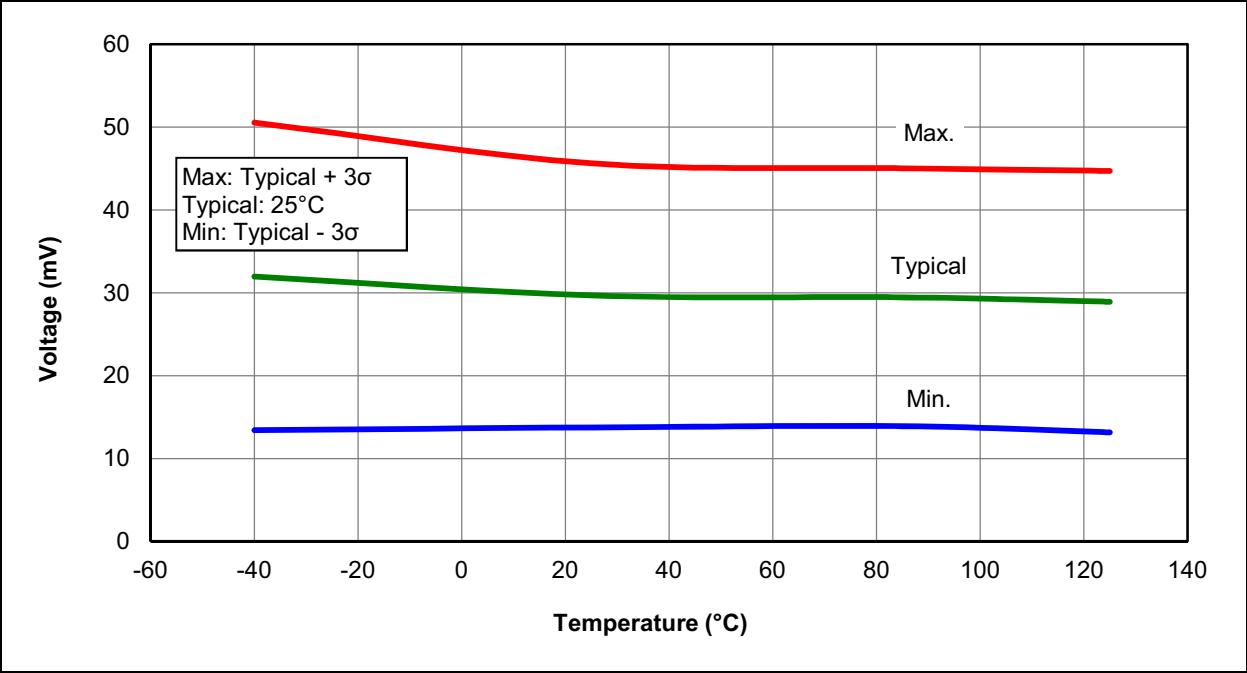
FIGURE 37-10: BROWN-OUT RESET HYSTERESIS, BORV = 1, PIC16LF1773/6 ONLY
