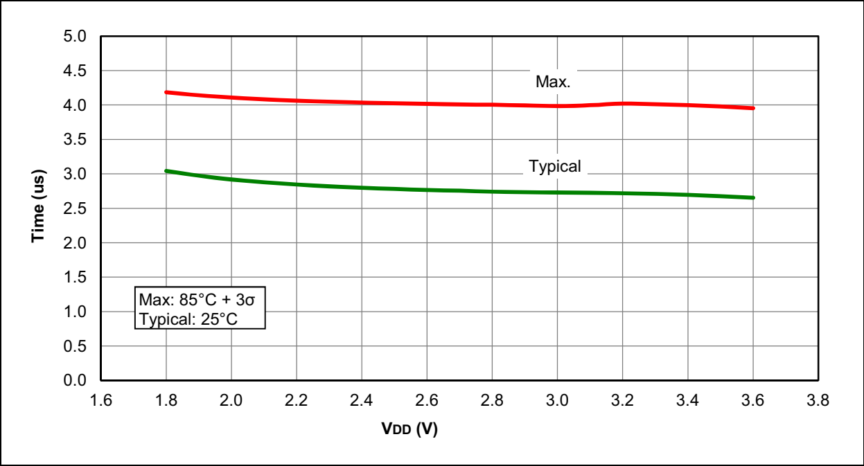
FIGURE 37-22: SLEEP MODE, WAKE PERIOD WITH HFINTOSC SOURCE, PIC16LF1773/6 ONLY
