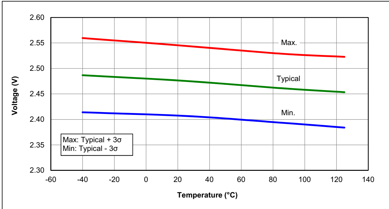
FIGURE 37-11: BROWN-OUT RESET VOLTAGE, BORV = 1, PIC16F1773/6 ONLY
