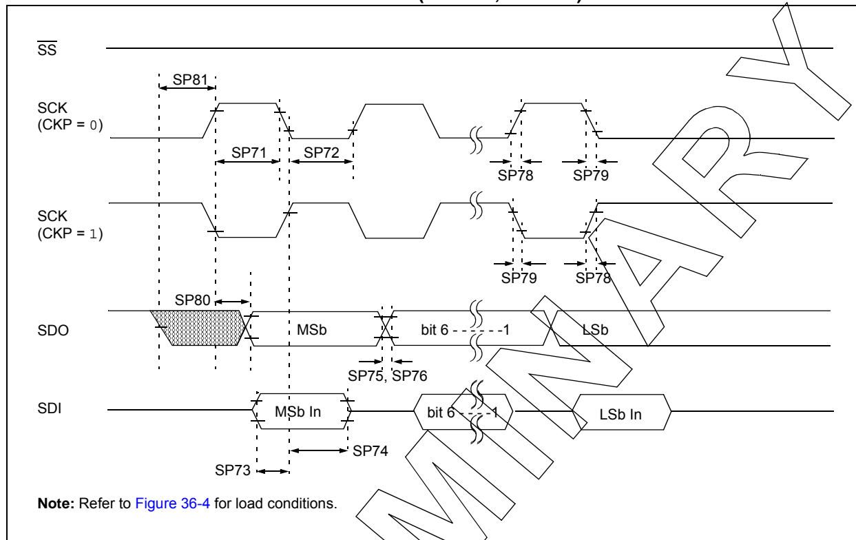
FIGURE 36-18: SPI MASTER MODE TIMING (CKE = 1, SMP = 1)
