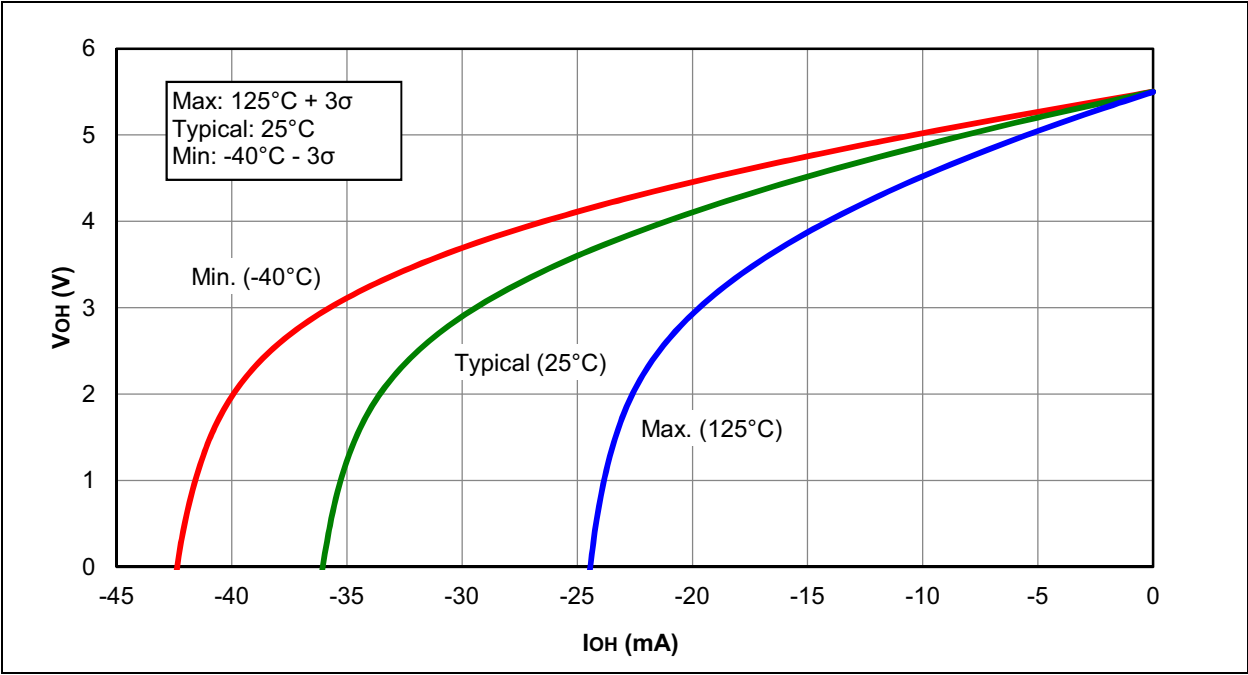
FIGURE 37-1: V_{OH} vs. I_{OH} OVER TEMPERATURE, V_{DD} = 5.5V , PIC16F1773/6 ONLY
