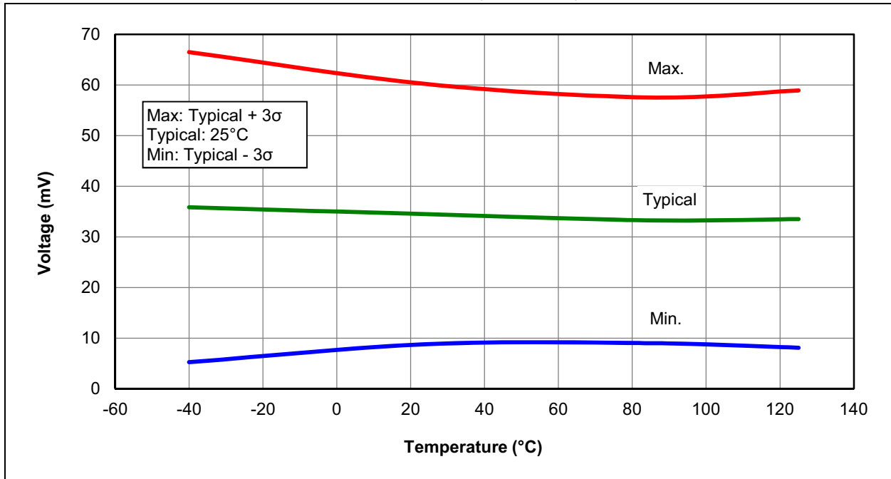
FIGURE 37-12: BROWN-OUT RESET HYSTERESIS, BORV = 1, PIC16F1773/6 ONLY
