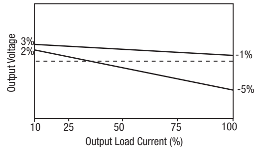
MGJ2D121505SC & MGJ2D241505SC
