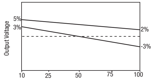
MGJ2D121505SC & MGJ2D241505SC
