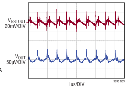
Transient Output Ripple
