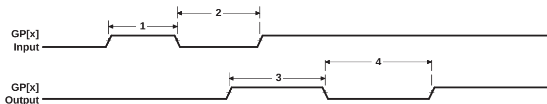
Figure 6-46. GPIO Port Timing
