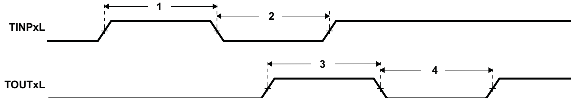
Figure 6-43. Timer Timing
