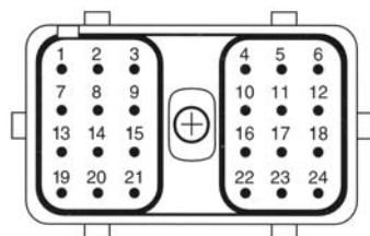
In-line Receptacle
