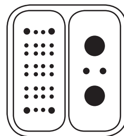
FL*-36A 2 - SRK Ø8mm 6 - Size 16 28 - Size 20
