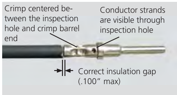
Acceptable Crimp
