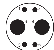
18-6 2 size 4 & 4 size 16 N, E
