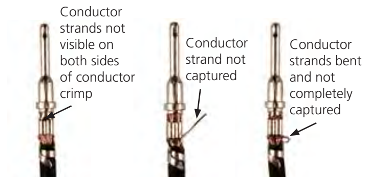
Unacceptable Crimps
