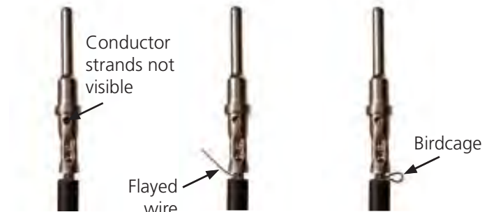
Unacceptable Crimps
