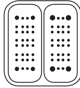
FL*-64A 8 - Size 16 56 - Size 20
