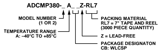
Figure 16. Ordering Code Structure
