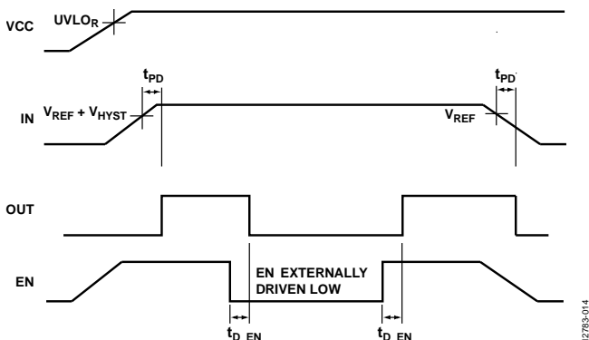
Figure 14. Timing Diagram
