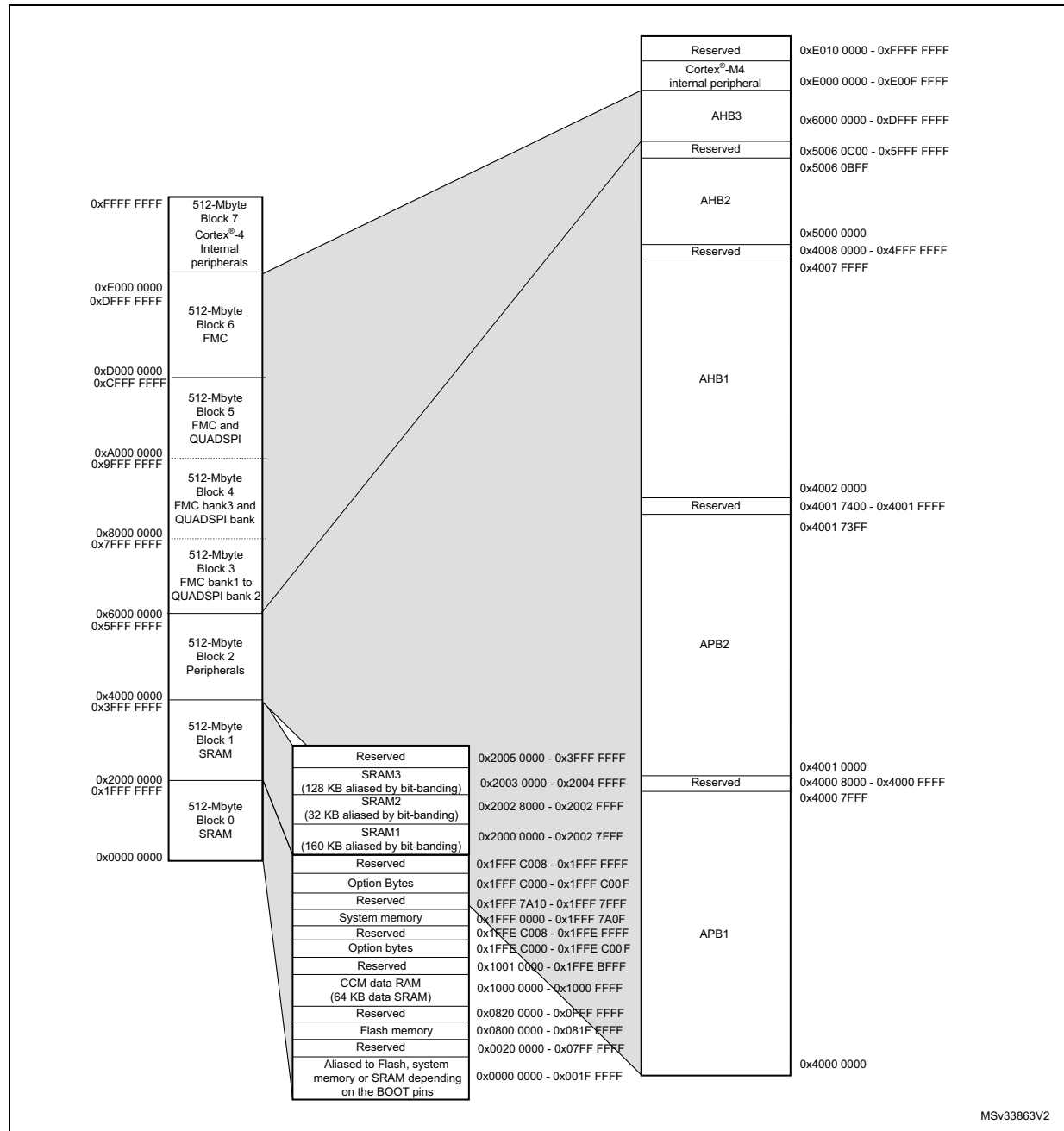
Figure 19. Memory map
