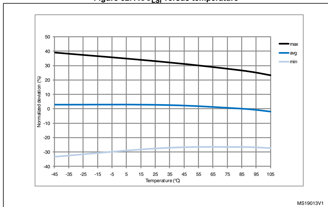
Figure 32. \text{ACC}_{\text{LSI}} versus temperature
