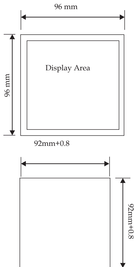
Panel Cutout
