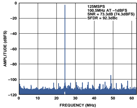
Figure 12. Single-Tone FFT with f_{IN} = 100.5 MHz
