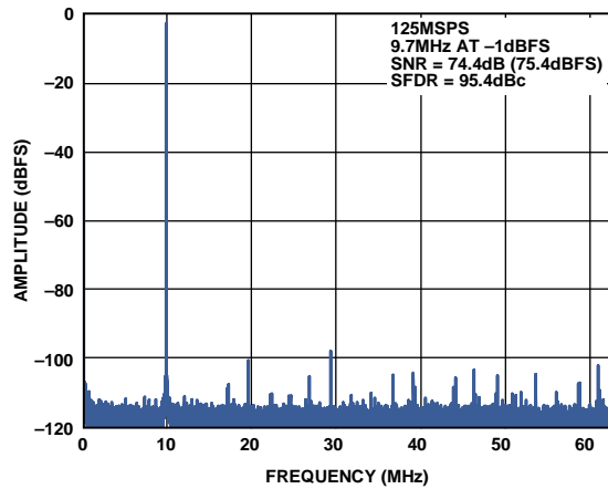
Figure 9. Single-Tone FFT with f_{IN} = 9.7 MHz
