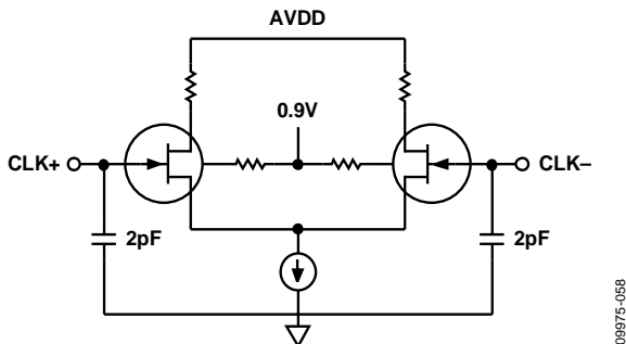
Figure 51. Equivalent Clock Input Circuit
