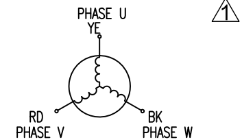
STAR CONNECTION
