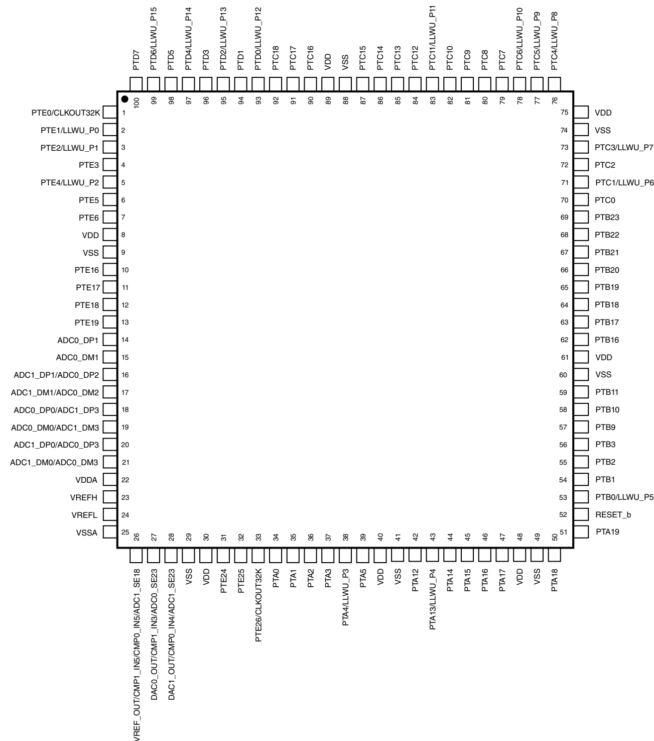
Figure 27. KV31F 100 LQFP Pinout Diagram (top view)
