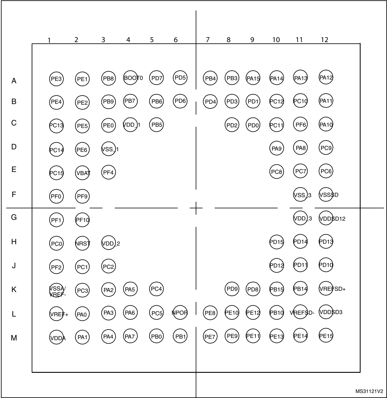
Figure 5. STM32F378xx BGA100 ballout
