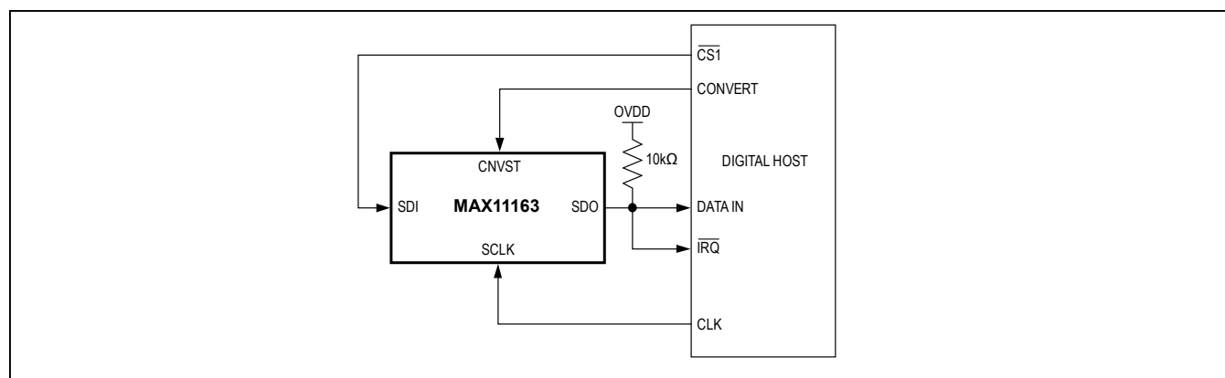
Figure 11. \overline{CS} Mode 4-Wire with Busy Indicator Connection Diagram
