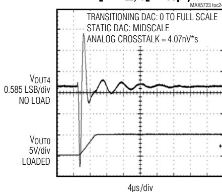
CHANNEL-TO-CHANNEL FEEDTHROUGH ( V_{DD} = V_{REF} = 5V , T_A = +25^\circ\text{C} , R_L = 2k\Omega , C_L = 200pF )
