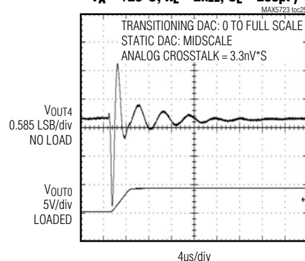
CHANNEL-TO-CHANNEL FEEDTHROUGH ( V_{DD} = 5V , V_{REF} = 4.096V (INTERNAL), T_A = +25^\circ\text{C} , R_L = 2k\Omega , C_L = 200pF )
