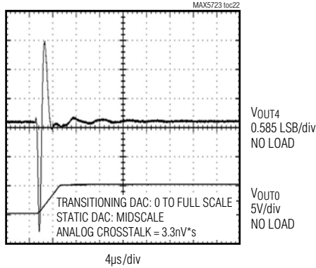
CHANNEL-TO-CHANNEL FEEDTHROUGH ( V_{DD} = V_{REF} = 5V , T_A = +25^\circ\text{C} , NO LOAD)
