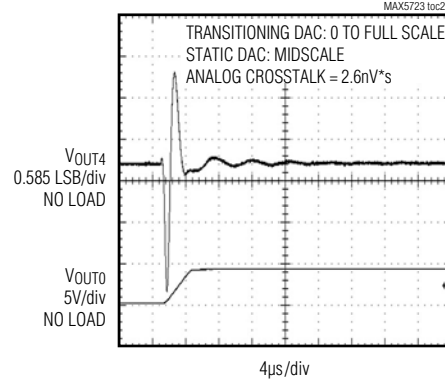
CHANNEL-TO-CHANNEL FEEDTHROUGH ( V_{DD} = 5V , V_{REF} = 4.096V , T_A = +25^\circ\text{C} , NO LOAD)
