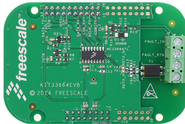
KIT33664EVB Evaluation Board
