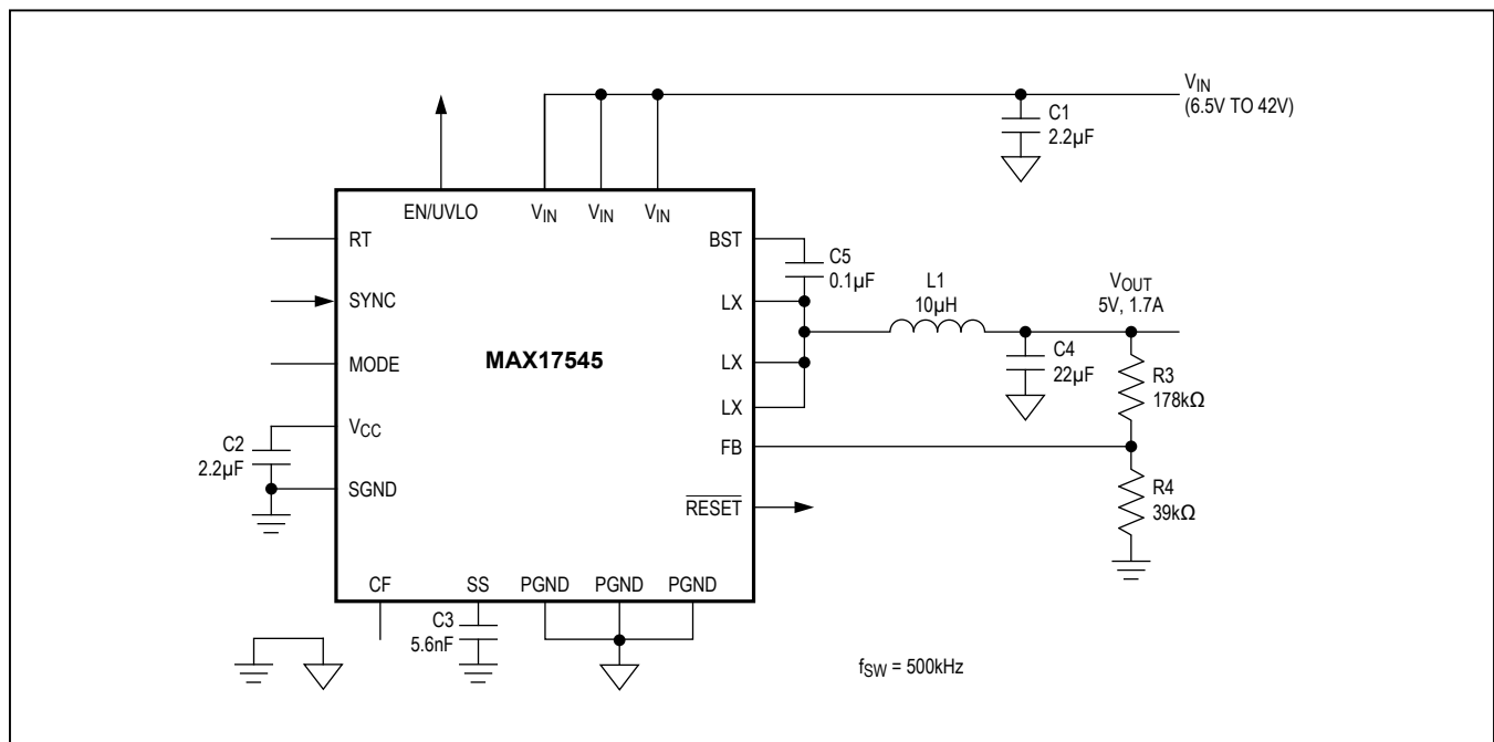
Figure 4a. 5V Output, 500kHz Switching Frequency
