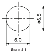
Recommended Mounting Hole
